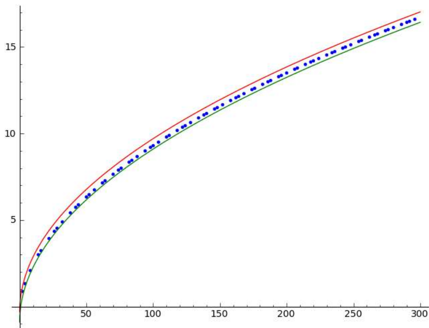
Figure 1: Support for Conjecture 1.2. Blue dots indicate points of the form (n, n^{1/2}(1 - \alpha_n)) . The red curve is x^{1/2} - .3 , and the green curve is x^{1/2} - .9 .
