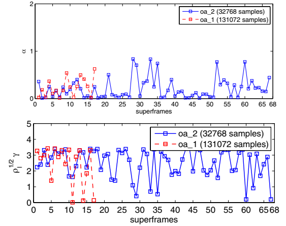
Fig. 5. Sampled values of the characteristic exponent \alpha and standard deviation \sqrt{\rho_l \gamma} of the SaS noise averaged across the iterations of the Gibbs sampler for each superframe (i.e., segment) in the overlap-and-add method.
