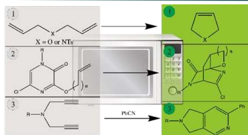
Figure 2. MAOS process for several organic reactions.
