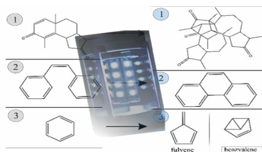
Figure 3. Photochemistry reaction for the production of organic compounds.
