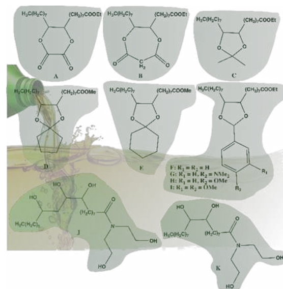
Figure 4. Structure of Biolubricant compound A-K.
