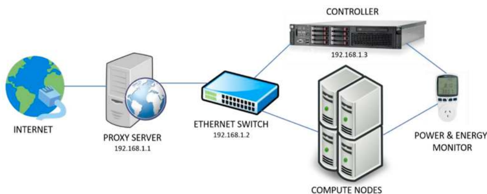
Figure 6. Experimental set-up.
