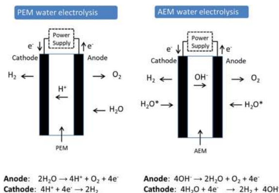
Fig. 1 Comparison of water electrolysis cells and chemistries using either a Proton Exchange Membrane (PEM) or an Anion Exchange Membrane (AEM). * Current AEM electrolysers use a water feed with added electrolyte (HCO 3 - /CO 3 2- or dilute KOH) to obtain sufficient performance. AEM electrolysers can operate with electrolyte feed at both electrodes or in anode feed only mode.
