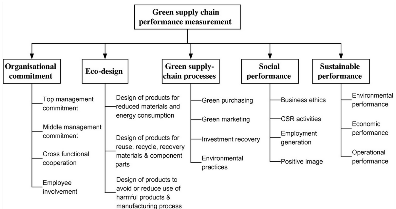
Figure 2 GSC constructs.
