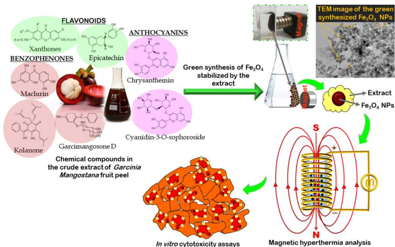
Figure 1 A schematic of the chemical compounds in the crude extract of G. mangostana fruit peel which served as a green stabilizer to synthesize Fe 3 O 4 NPs for magnetic hyperthermia study and elimination of the colon cancer cells.
