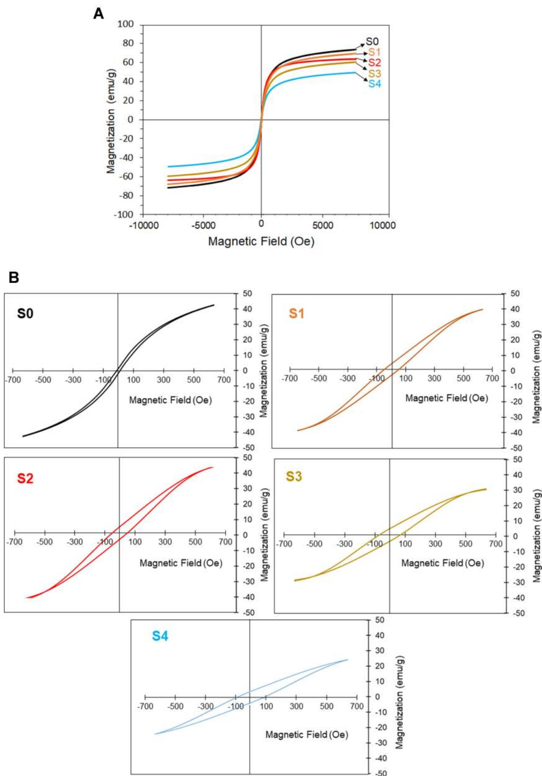
Figure 5 (A) Saturation magnetization and (B) coercivity of the synthesized Fe 3 O 4 NPs (S0–S4).
