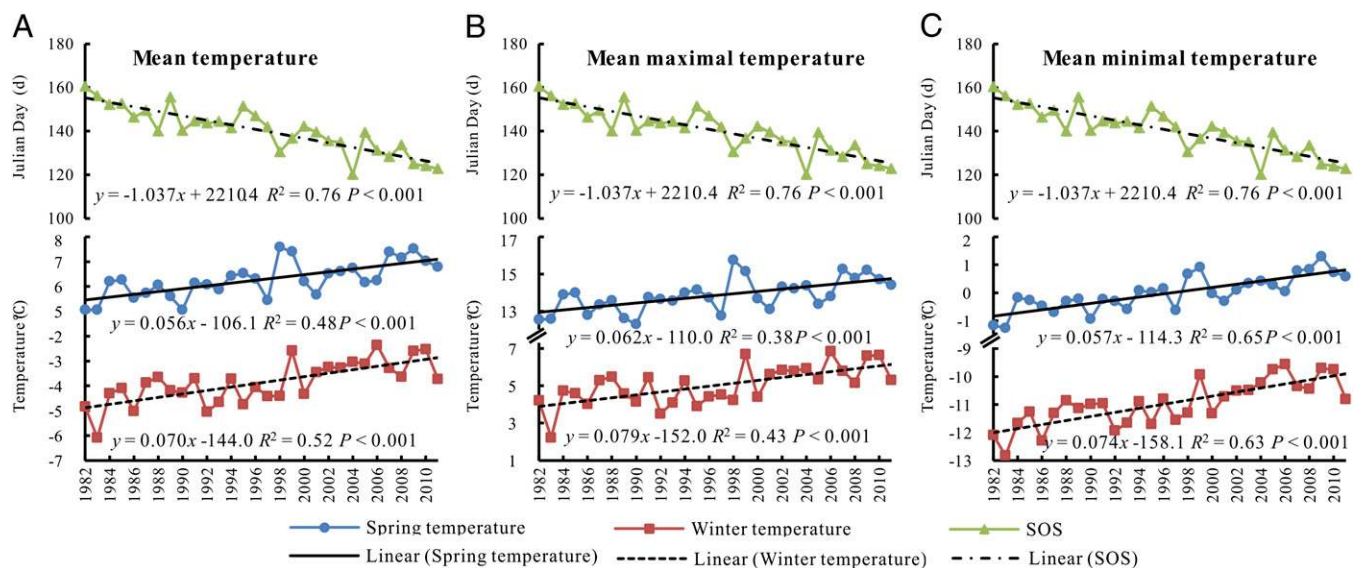
Fig. 4. Interannual variations in mean temperature (A), mean maximal temperature (B), and mean minimal temperature (C) in winters (from November of the prior year to March of the following year) and springs (April and May) and vegetation SOS integrating GIMMS-based SOS (1982–2000) and SPOT-VGT-based SOS (2001–2011) from 1982 to 2011 in the Tibetan Plateau. The correlation coefficients between the SOS and the mean temperature in springs and winters, the mean maximal temperature in springs and winters, and the mean minimal temperature in springs and winters are -0.7052 and -0.7029 , -0.6718 and -0.6704 , and -0.7591 and -0.7313 , respectively. All correlation coefficients are significant at the 0.001 level.
