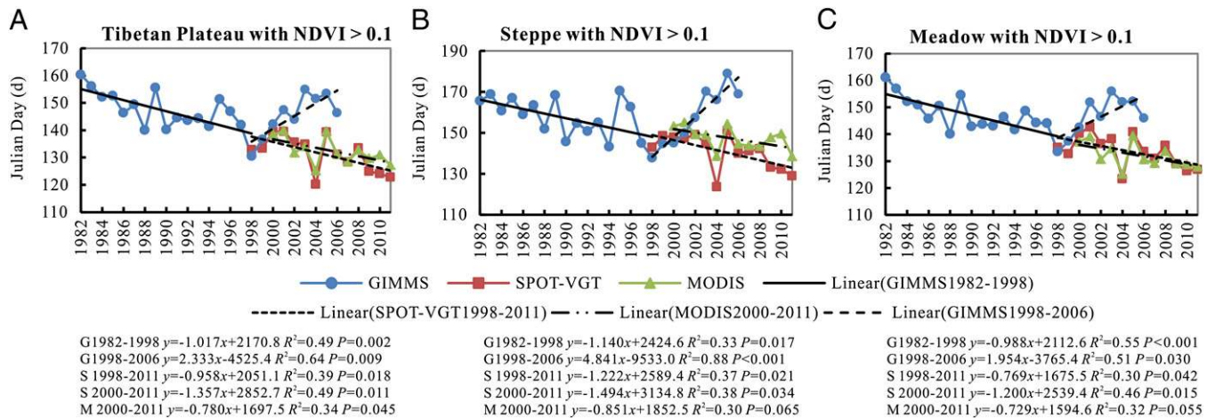
Fig. 1. Interannual variations in vegetation SOS from 1982 to 2011 based on the GIMMS (1982–2006), SPOT-VGT (1998–2011), and MODIS (2000–2011) NDVI datasets in the whole Tibetan Plateau region (A), alpine steppe region (B), and alpine meadow region (C). Note: alpine steppe and alpine meadow are the primary vegetation types in the plateau. The formulas show the linear fitting functions of the green-up dates and year. G, S, and M before the formulas are the abbreviations for the GIMMS, SPOT-VGT, and MODIS datasets, respectively.
