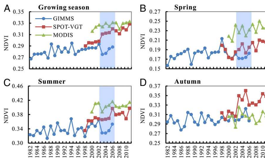
Fig. 2. Interannual variations in NDVI over the entire Tibetan Plateau during the growing season (A), spring (B), summer (C), and autumn (D) based on the GIMMS (1982–2006), SPOT-VGT (1998–2011), and MODIS (2000–2011) datasets. During the growing season, the slopes of the increasing trend based on the GIMMS, SPOT-VGT, and MODIS NDVI datasets are 4.64 \times 10^{-4} \text{ y}^{-1} ( R^2 = 0.21 , P = 0.021 , n = 25 ), 26.56 \times 10^{-4} \text{ y}^{-1} ( R^2 = 0.87 , P < 0.001 , n = 14 ), and 9.14 \times 10^{-4} \text{ y}^{-1} ( R^2 = 0.40 , P = 0.028 , n = 12 ), respectively. The correlation coefficients between the SPOT-VGT and MODIS NDVI in growing season, spring, summer, and autumn during their overlapping period (2000–2011) are 0.7440 ( P = 0.005 ), 0.8469 ( P < 0.001 ), 0.6300 ( P = 0.028 ), and 0.5968 ( P = 0.041 ), respectively. The gray pillars show the time range with abnormal GIMMS data.
