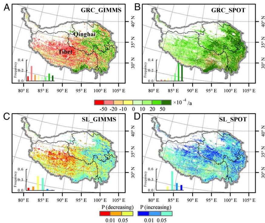
Fig. 3. Spatial distributions of the greenness rate of change (GRC) (A and B) and significance levels (SL) (C and D) of the NDVI change in the Tibetan Plateau during the growing season from 1998 to 2006 based on the GIMMS and SPOT-VGT datasets. P(\text{decreasing}) and P(\text{increasing}) are the P values of the decrease and increase in the growing season NDVI, respectively, which are divided into three levels: P < 0.01 , 0.01 < P < 0.05 , and P > 0.05 . The insets show the frequency distributions of corresponding trends (A and B) and different significance levels (C and D).
