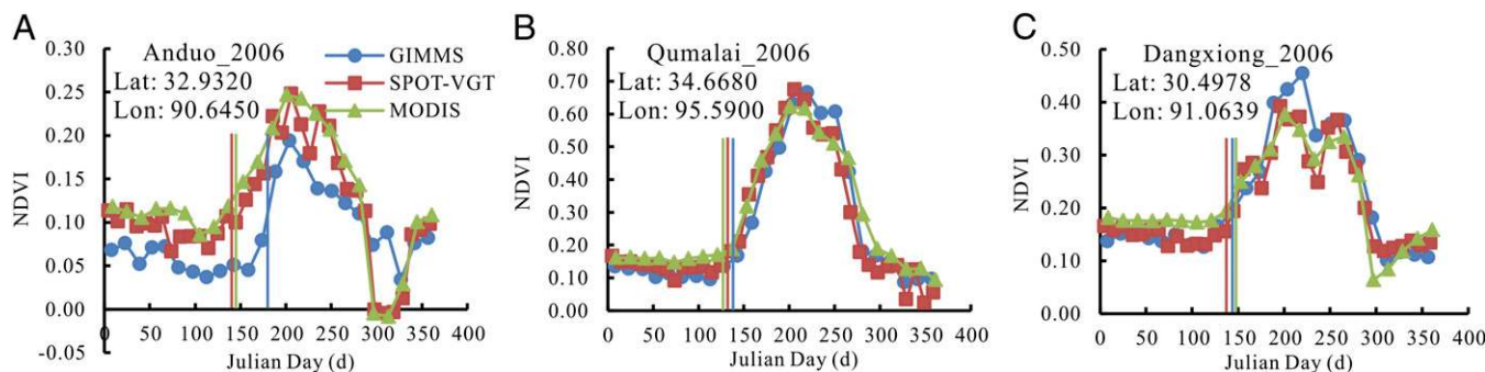
Fig. 5. Vegetation growth curves in the three sampled sites in 2006 (A, Anduo; B, Qumalai; and C, Dangxiong) based on the GIMMS, SPOT-VGT, and MODIS NDVIs. The blue, red, and green straight lines show the retrieved vegetation SOS dates based on GIMMS, SPOT-VGT, and MODIS NDVIs, respectively. The NDVIs were averaged over a round area with a 5-km radius centered on each site. These dates are calculated by the SOS retrieval method ( Materials and Methods ).
