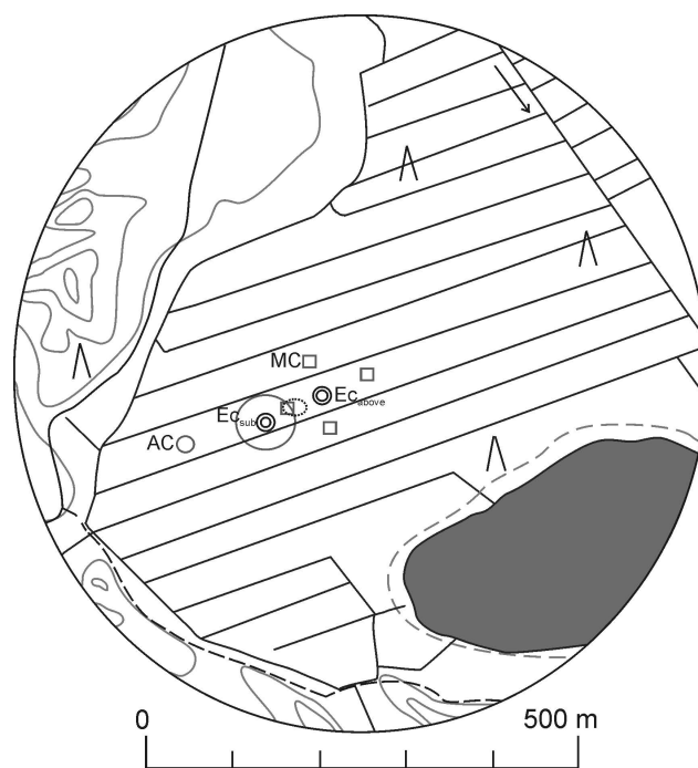
Fig. 1. Map of the measurement site showing the locations of above canopy eddy covariance (EC) mast (EC above ), sub-canopy EC mast (EC sub ), manual chambers (MC, square) and automatic chambers (AC, circle). Dotted line next to one of the manual chamber groups show the place of soil gas concentration pits, and grey line around the sub-canopy EC mast show the footprint area from which 85% (at 30 m) of the sub-canopy N 2 O fluxes originate (see Mammarella et al., 2010).
