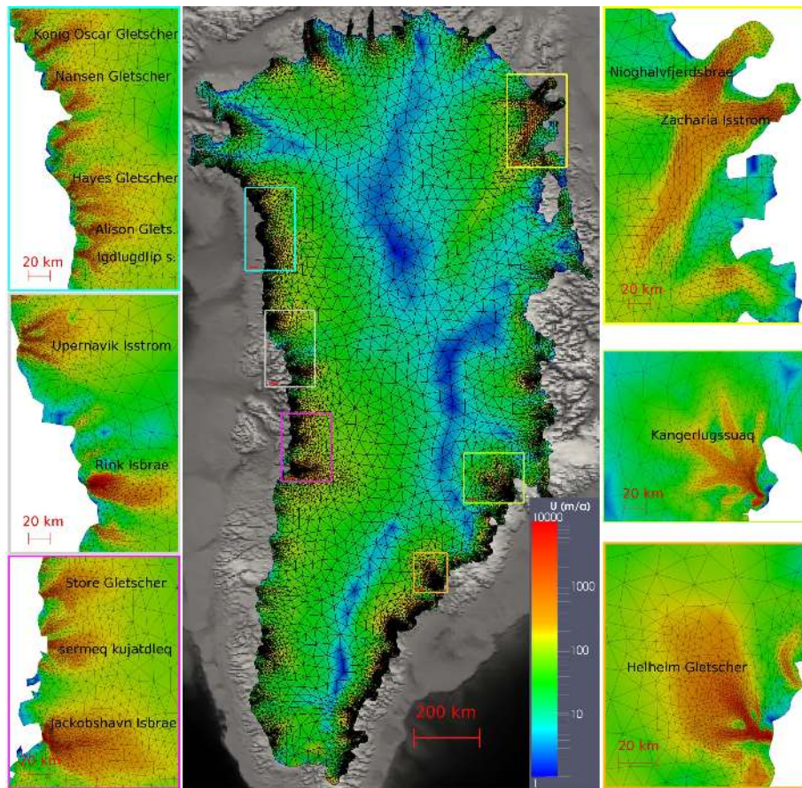
Fig. 2. Unstructured finite element mesh and model surface velocities after optimisation of the basal friction coefficient with the Robin inverse method. Colored boxes show close-up views for various outlet glaciers of interest.
