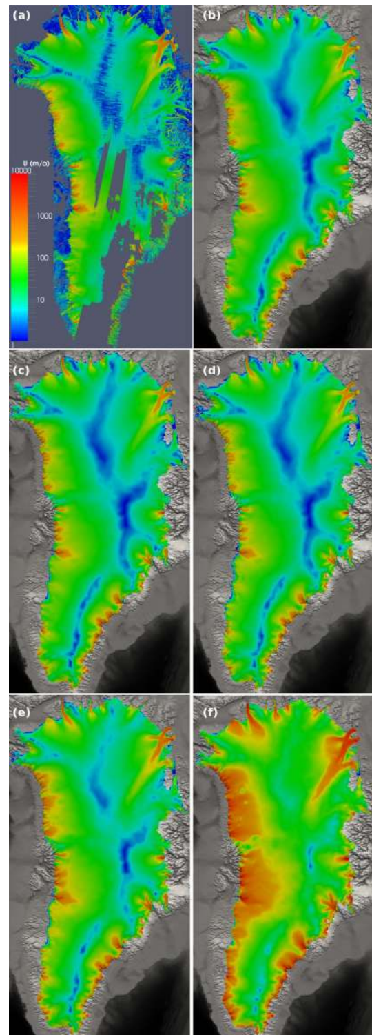
Fig. 1. GrIS surface velocities. (a) Observed surface velocities on the original regular 500\text{m} \times 500\text{m} grid; Computed surface velocities: (b) after relaxation; after one century for (c) experiment C1_BF1, (d) experiment C2_BF1, (e) experiment C2_BF2 and (f) experiment C2_BF3.
