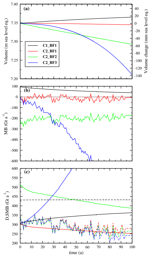
Fig. 8. GrIS future mass balance as a function of time: (a) total ice volume (left axis, meters of sea level equivalent) or volume change from initial time (right axis, millimeters of sea level equivalent), (b) annual mass balance (the brown line correspond to 0) and (c) discharge ( D ) (solid lines) and SMB (dashed lines) in \text{Gt a}^{-1} .
