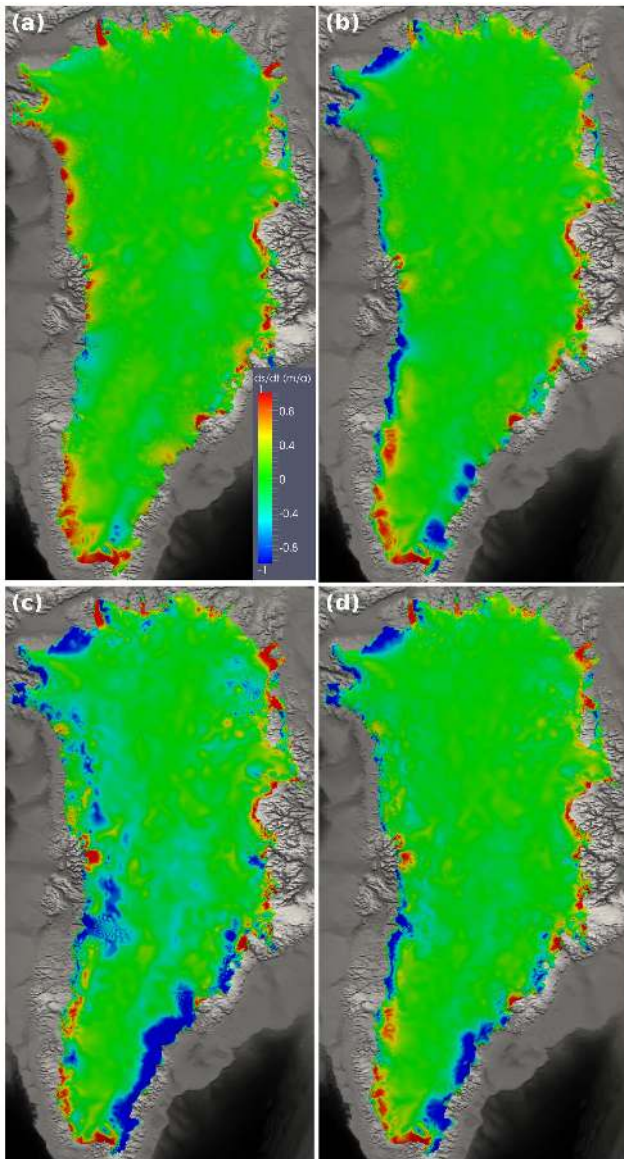
Fig. 9. Free surface elevation rate of change after 10 yr for experiments (a) C1.BF1, (b) C2.BF1, (c) C2.BF2, and (d) C2.BF3.
