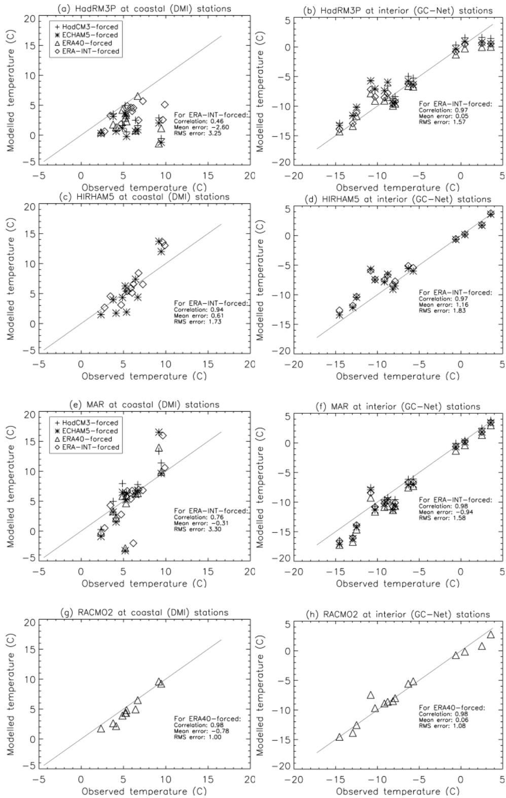
Fig. 2. 20-yr mean modelled versus observed summer (JJA) T_{as} ( ^{\circ}\text{C} ). Each point represents an observing station. The line of 1 : 1 correspondence is also shown. The legend, given in (a), is the same in all figures. Correlations between modelled and observed 20-yr mean T_{as} , and the mean and RMSEs of the model output relative to observations, are also given for the ERA-Interim-forced HadRM3P, MAR and HIRHAM5 simulations, and the ERA40-forced RACMO2 simulation.
