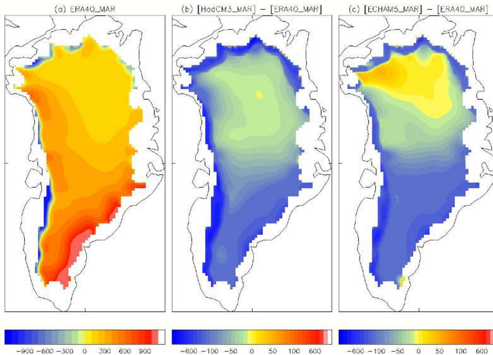
Fig. 8. 1980–1999 mean surface mass balance (SMB), in \text{mm w.e. yr}^{-1} . (a) ERA40-forced MAR. (b) Difference between HadCM3-forced MAR and ERA40-forced MAR. (c) Difference between ECHAM5-forced MAR and ERA40-forced MAR.
