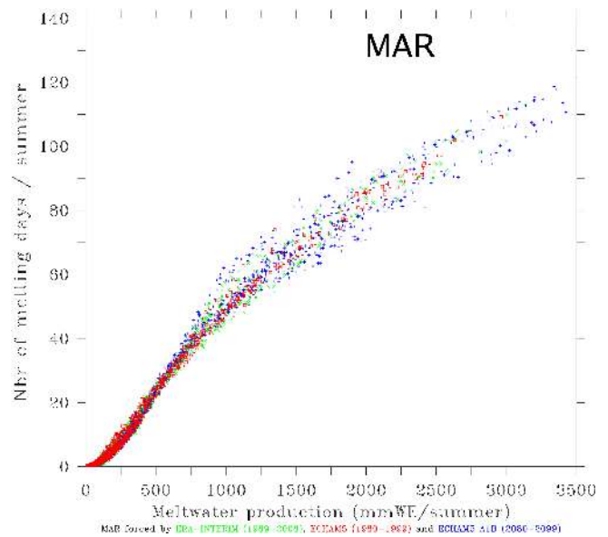
Fig. 12. Scatter plot of the mean number of melt days versus the mean annual meltwater production (in mm\ w.e.\ yr^{-1} ), for each grid box and for each year of simulation, for MAR forced by ERA-Interim over 1989–2008, ECHAM5 (recent past) over 1980–1999 and ECHAM5-A1B over 2080–2099.
