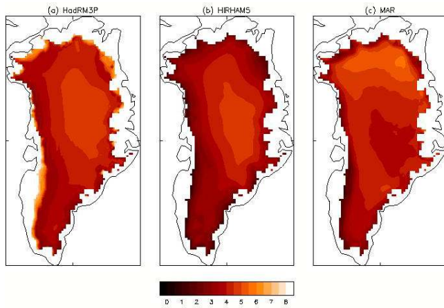
Fig. 11. 2080–2099 T_{as} anomalies ( ^{\circ}C ), relative to 1980–1999, over the GrIS in ECHAM5-A1B-forced simulations. (a) HadRM3P, (b) HIRHAM5, (c) MAR.
