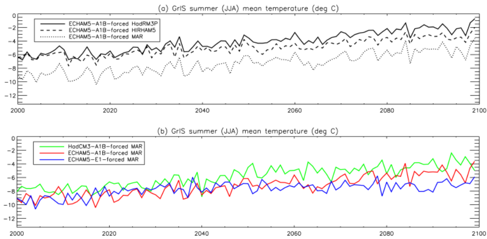
Fig. 10. (a) Time series of GrIS mean summer (JJA) T_{as} , all in ^{\circ}C , for the three RCMs, forced by ECHAM5-A1B boundary conditions. (b) Similar, for MAR, forced by all three sets of future boundary conditions.
