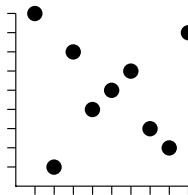
Figure 2: The plot of the skew-merged permutation 917456328.
