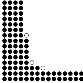
Figure 1: The plot of downset in \mathbb{N}^2 ; the elements of the class are drawn with solid circles, while the elements of the basis are drawn with hollow circles.
