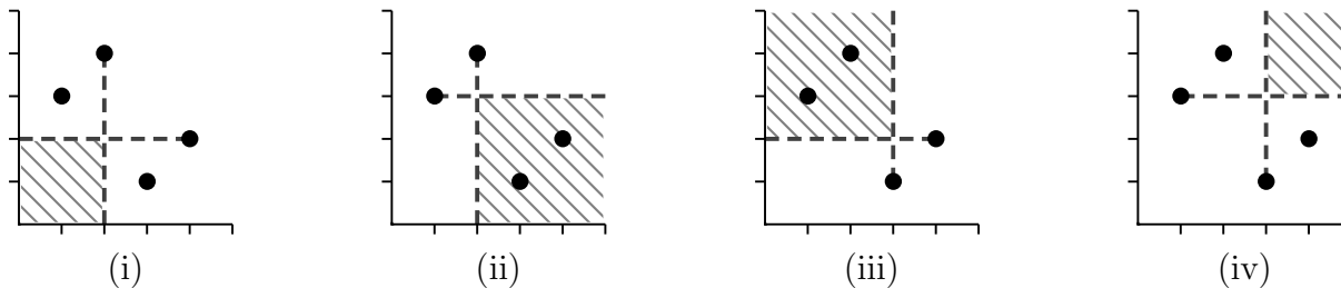
Figure 4: The regions of \pi referred to in the proof of Theorem 2.5.
