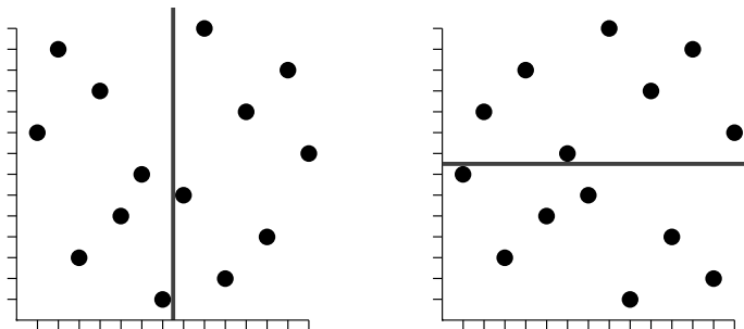
Figure 6: A horizontal alternation (left) and its inverse, a vertical alternation (right).
