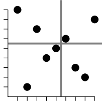
Figure 3: A gridding of the skew-merged permutation 917456328.
