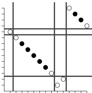
Figure 5: A greedy gridding of a permutation, showing its peg points as hollow circles; the peg permutation for this permutation is 5431276 while its non-peg vector is (0, 5, 0, 2) . Note that since this is a greedy gridding, the (1, 3) entry of the corresponding matrix must be 1.
