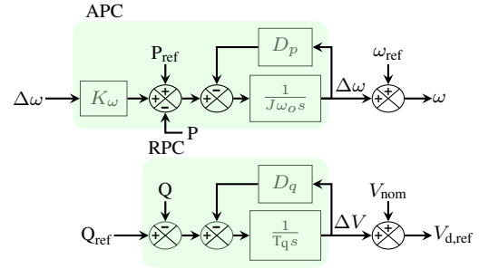
FIGURE 8. Simplified swing-based virtual synchronous generator.
