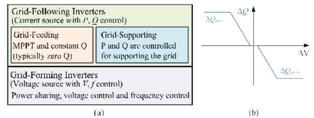
FIGURE 1. (a) Classification of grid-connected inverters and (b) reactive power control for supporting the grid.
