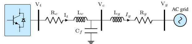
FIGURE 3. The power stage of a GFMI.
