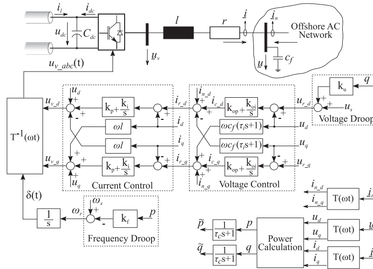
FIGURE 14. Grid forming HVDC system for an offshore AC network [143] (Copyright © 2018, IEEE).
