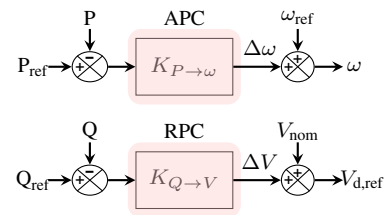
FIGURE 5. Droop controller.
