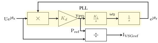
FIGURE 9. PLL that resembles a generator [42].
