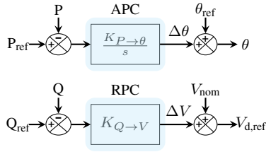
FIGURE 7. Power synchronization controller.
