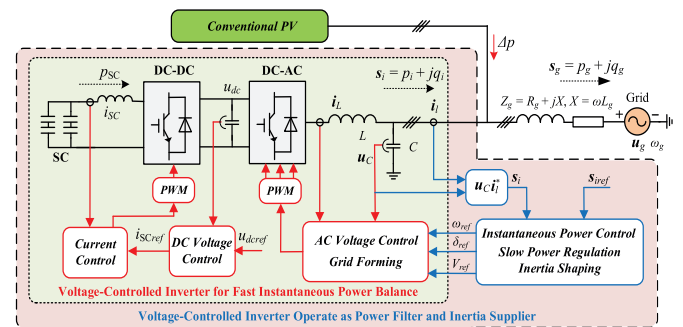
FIGURE 16. Schematic of the PVSG grid forming inverter [153] (Copyright © 2020, IEEE).
