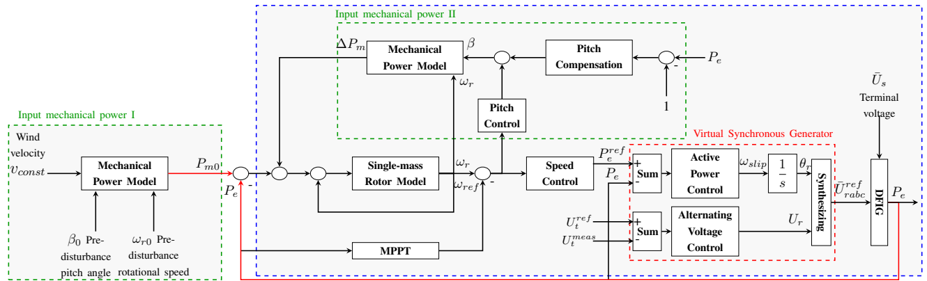
FIGURE 15. Control scheme for a DFIG-based WT with VSynC [147].
