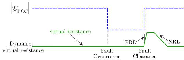
FIGURE 13. Dynamic virtual resistor for post-fault oscillation damping [96].
