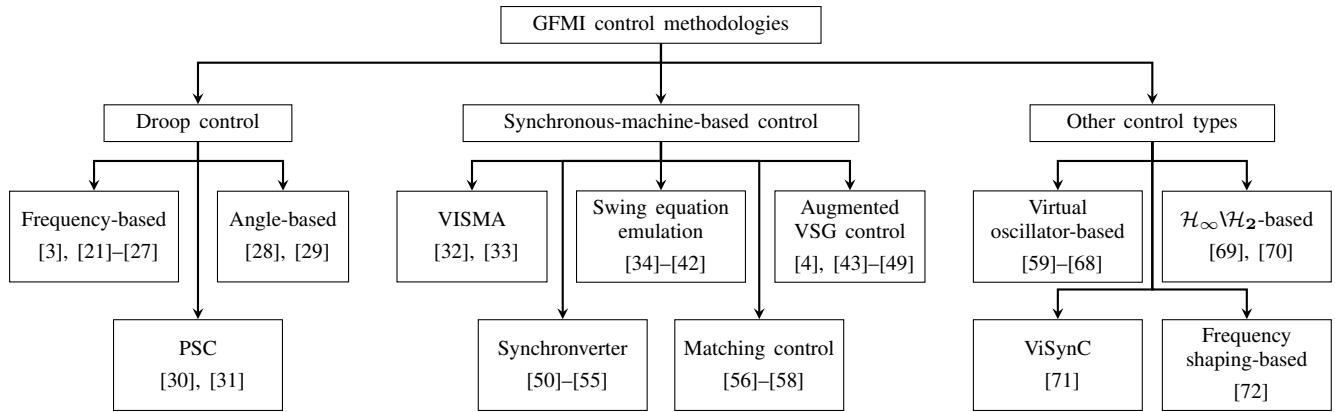
FIGURE 4. GFMI control methodologies.
