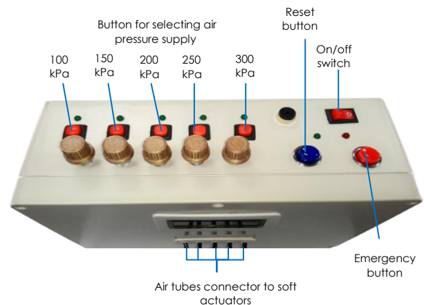
Figure 6 Control box
