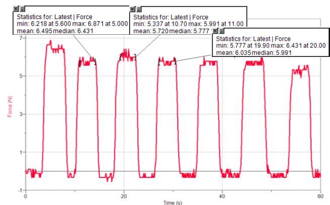
Figure 9 Grip forces measured at 200 kPa supplied air pressure of Subject 1's right hand.
