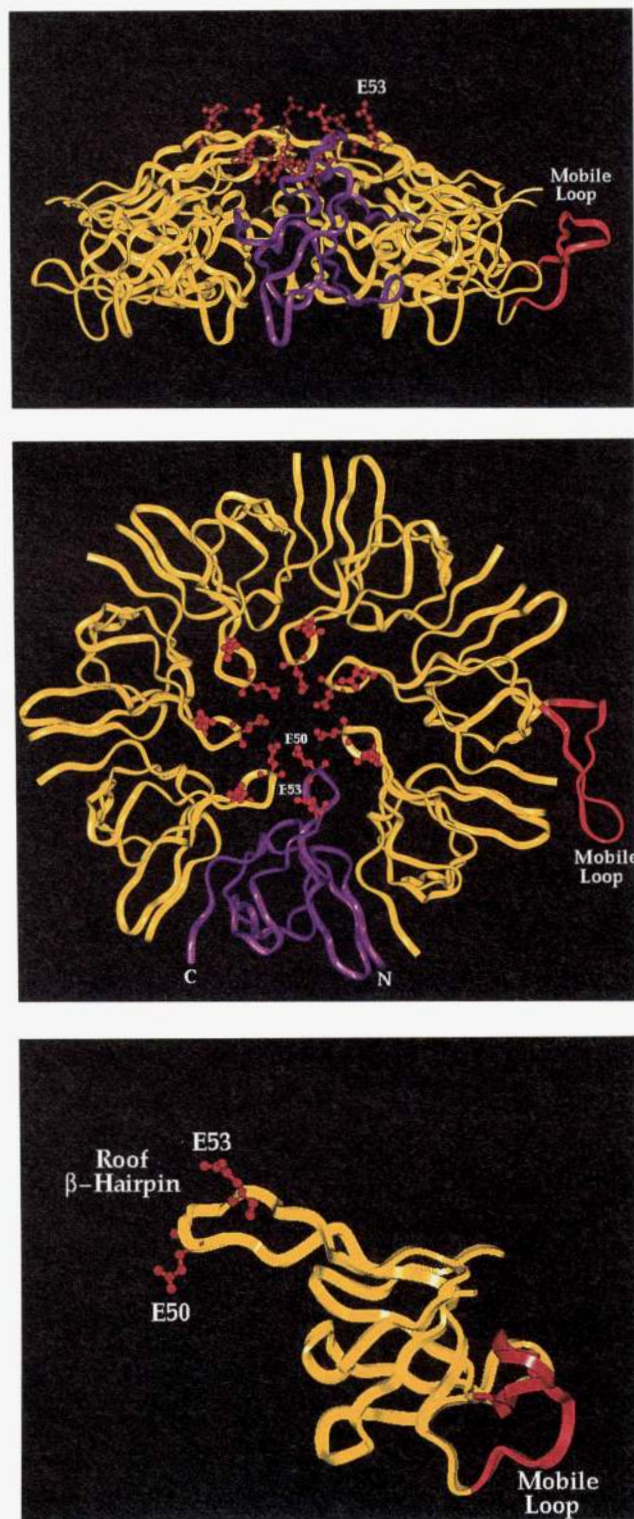
Fig. 2. GroES architecture. Side (upper panel) and top (center panel) orthogonal views of the GroES heptamer as a ribbon diagram (yellow). One subunit is shown in purple, and the single resolved mobile loop is shown in red. Also in red are ball-and-stick representations of the roof \beta -hairpin glutamates, E50 and E53. The amino (N) and carboxyl (C) termini of the purple subunit are indicated. In the lower panel, the monomer of GroES with the resolved mobile loop is shown, colored similarly. This view is rotated about 45° relative to that of the same subunit in the upper panel to show the central barrel and roof \beta -hairpin clearly. From Fenton et al. (1996), with permission.
