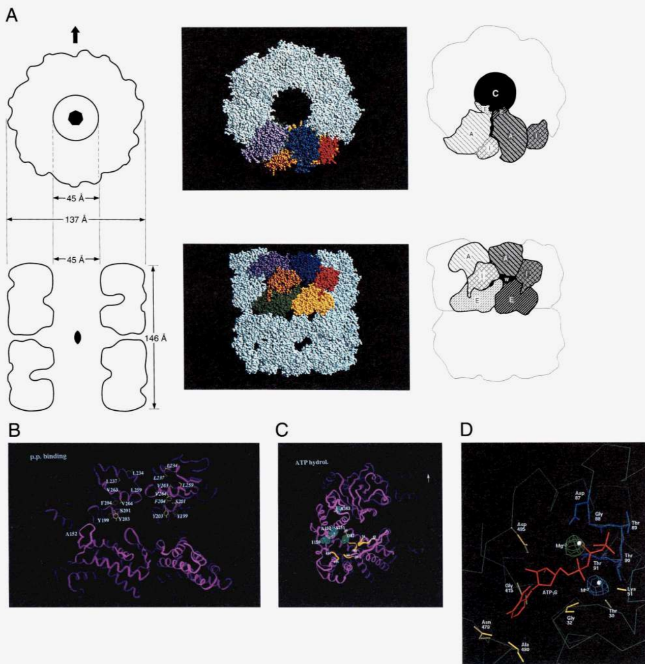
Fig. 1. GroEL architecture. A: The overall structure of the GroEL tetradecamer is shown in two views: from the top, looking into the central cavity; and from the side. The left panel gives the dimensions of the cylinder. The middle panel is a van der Waals space-filling model of the chaperonin, with two of the subunits in the upper ring colored to show the three domains, apical, intermediate, and equatorial: left subunit, purple, gold, green; right subunit, blue, red, yellow, respectively. The right panel is a diagrammatic representation of the middle one, with the domains designated A (apical), I (intermediate), and E (equatorial); also identified here are the central cavity (C) and one of the side openings (W). From Braig et al. (1994), with permission. B: Residues in the channel face implicated in polypeptide and GroES binding (side chains in yellow) are shown for two GroEL subunits, superimposed on ribbon diagrams of the backbone \alpha -carbon trace (purple). The view is from inside the central channel of the top ring in A; one subunit's residues are denoted in italics. From Fenton et al. (1994), with permission. C: ATP binding site and residues affecting ATP hydrolysis (green van der Waals spheres) are shown in a side view of a single subunit (purple backbone ribbon) from the upper ring; the central channel is to the right, outside is to the left. Residues around the binding pocket that are conserved are shown with small numbers and yellow coloring of the backbone. From Fenton et al. (1994), with permission. D: High-resolution view of the ATP binding site is shown, with ATP \gamma S (red) as the ligand. The backbone \alpha -carbon trace is cyan, residues involved in the phosphate binding loop are shown with side chains in dark blue, and other residues interacting with the nucleotide or the second cation are in yellow. The two cations are shown as white spheres, with the anomalous difference contour for Mg ^{2+} shown in green and the electron density contour for the second cation (M ^{2+} ) shown in light blue. Figure courtesy of D. Boisvert.
