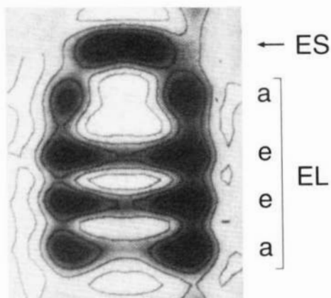
Fig. 3. GroEL–GroES binary complex. A section through the three-dimensional map of the asymmetric GroEL–GroES complex, generated by cryo-electron microscopy and image averaging, is shown. Apical (a) and equatorial (e) domains of GroEL (EL) are indicated. Note the difference in volume between the upper channel space under GroES (ES) and the lower unliganded channel. Redrawn from Chen et al. (1994), with permission.
