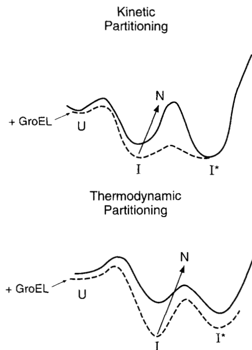
Fig. 5. Effects of GroEL on polypeptide folding intermediates. Two reaction coordinate diagrams are shown for the separate models of kinetic partitioning (top panel) and thermodynamic partitioning (lower panel). In both, U is the unfolded state, I is an intermediate state on the folding pathway, I* is a misfolded state, and N is the native protein; the angled arrow from I to N is meant to imply folding along another coordinate in three-dimensional space. The solid line indicates the absence of GroEL and the dashed line, its presence. In kinetic partitioning, the major effect of GroEL is to lower the transition state between I* and I , whereas for thermodynamic partitioning, the effect is to increase the stability of I relative to I* (see text for details).
