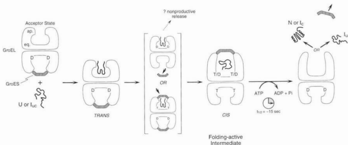
Fig. 4. Model for a GroEL–GroES-mediated folding reaction. The asymmetric GroEL–GroES complex (first panel: ap., apical domain; eq., equatorial domain) is the likely polypeptide acceptor state in vivo , and binds unfolded polypeptides ( U ) or kinetically trapped folding intermediates ( I uc ) to form the trans ternary complex (second panel). This complex is highly dynamic with respect to GroES binding in the presence of ATP; two of the possible pathways of GroES release and rebinding that lead to the cis complex are shown (third panel). When polypeptide is sequestered underneath GroES in the presence of ATP (the folding-active cis intermediate, fourth panel), major conformational changes occur in the cis GroEL ring, and polypeptide folding is initiated. Simultaneously, ATP binding in the trans ring starts the timer for hydrolysis and release. When ATP hydrolysis occurs in the trans ring ( t_{1/2} \sim 15 s), GroES is released, giving polypeptide the opportunity to depart (last panel). The released polypeptide is either native ( N ) or committed to fold ( I c ), or is in an uncommitted or kinetically trapped state ( I uc ), which can rebind to the same or a different GroEL complex and undergo another cycle of folding. In the complexes, D designates ADP and T, ATP. Redrawn from Fenton et al. (1996), with permission.
