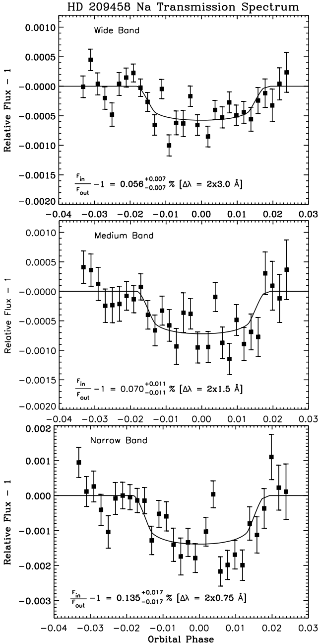
Fig. 4. Transit photometry averaged in two bands centered on the Na D doublet, with spectral widths of 3 \text{ \AA} (top panel), 1.5 \text{ \AA} (middle panel) and 0.75 \text{ \AA} (bottom panel). The data have been empirically corrected for the dependence of the depth of stellar lines on the count level in the spectra, as discussed in detail in Sect. 2.1.
