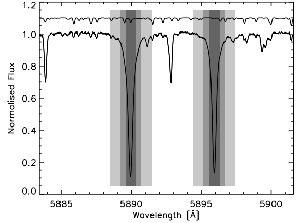
Fig. 1. Spectrum of HD 209458 around the NaD doublet. The shaded areas indicate the narrow, medium, and wide passbands as used in our analysis. In all cases, the comparison bands are located directly adjacent to the central band, and have the same width. The upper line shows a synthetic telluric spectrum constructed from the line list of Lundstrom et al. (1991). Note that the telluric sodium absorption can show strong seasonal variability.
