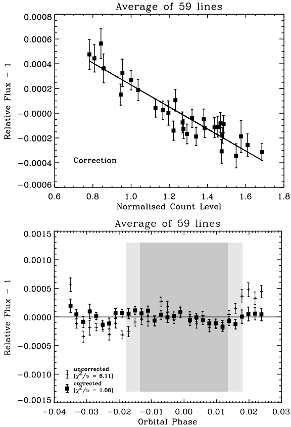
Fig. 3. The top panel shows the normalized count level of the continuum in the spectra versus the measured weighted mean-strength of 59 deep stellar absorption lines. A strong inverse correlation is present, with the more flux in the spectra, the deeper the absorption lines. We believe that this is due to a non-linearity effect in the CCD. The solid line indicates the linear least squares fit to the correlation, used to correct the measured line strengths. The lower panel shows the same average strength of these 59 absorption lines as function of orbital phase, where the grey band indicates the planetary transit. Those data points corrected for the correlation with count level (thick squares) have a reduced chi-squared of 1.06, while the uncorrected data exhibit a reduced chi-squared of 6.11.
