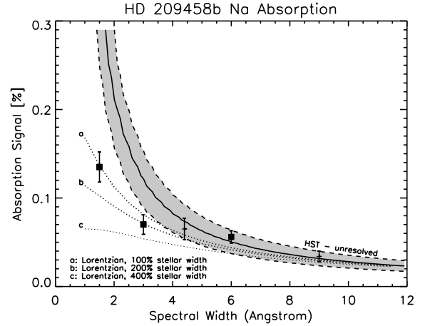
Fig. 5. The three measurements of the Na D absorption in the transmission spectrum of HD 209458b in passbands of 2 \times 0.75 \text{ \AA} , 2 \times 1.5 \text{ \AA} , and 2 \times 3.0 \text{ \AA} . The solid line and grey band indicate the HST measurement by Charbonneau et al. (2002) assuming it is completely unresolved and within our passbands. The three dotted lines, indicated by a , b , c , are the Na D absorption levels as a function of passband expected from the HST measurements, assuming that the atmospheric absorption feature is Lorentzian shaped with a width equal to, 2\times , and 4\times the stellar width of the Na D doublet. The two crosses at 4.4 and 9 \text{ \AA} are the results from the re-analysed STIS/HST data by Sing et al. (2008a).
