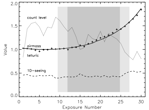
Fig. 2. Variations of observing conditions over the 30 spectra. The solid line indicates the airmass, and the dotted line shows the normalised variation in continuum count level. The dashed line indicates the seeing (in \sigma ) as measured from the one-dimensional profile of the star along the slit. The crosses show the relative telluric line strength as measured using strong lines in the red part of the spectrum. It follows the airmass well, implying that the conditions were excellent. The grey band indicates the timing of the planetary transit and periods of ingress and egress.
