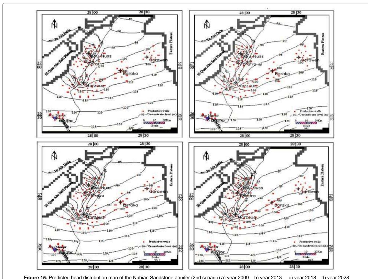
Figure 15: Predicted head distribution map of the Nubian Sandstone aquifer (2nd scenario) a) year 2009 b) year 2013 c) year 2018 d) year 2028
