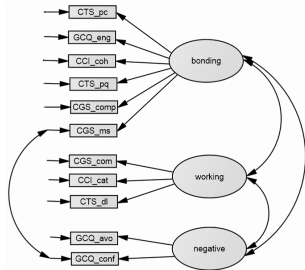
Figure 1. The first model fit statistics. Chi-squared: 44.31, df = 41 . Comparative fit index: .976. RMSEA: .017. p for test of close fit: .788.
