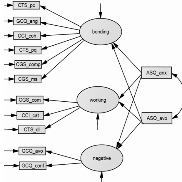
Figure 3. The hypothesized third model fit statistics. CGS = Cohesion Group Scale; GCQ = Group Climate Questionnaire; CCI = Curative Climate Inventory; CTS = Cohesion Therapist Scale; ASQ = Attachment Styles Questionnaire, ms = mutual stimulation; eng = engagement, coh = cohesion, pq = positive qualities; comp = compatibility; pc = personal compatibility; com = commitment, cat = catharsis; dl = dissatisfaction role leader; conf = conflict; avo = avoiding, anx = anxiety.
