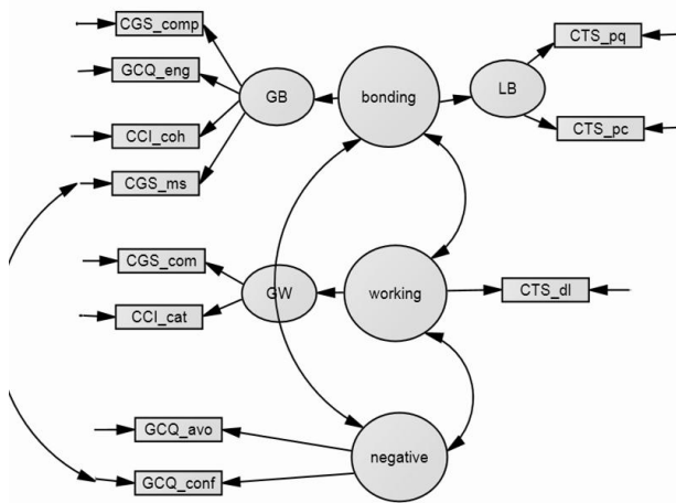
Figure 2. The second model fit statistics. Chi-squared 45.09; df = 39; comparative fit index: .954, RMSEA: .039, p for test of close fit: .364.
