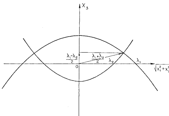
FIG. 3. Parabolic coordinates.
