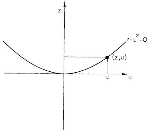
FIG. 4. Projection of a p -dimensional space on a paraboloid in p+1 dimensions.
