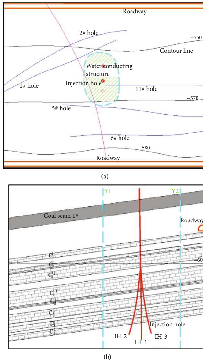
FIGURE 10: Grout holes in engineering. (a) Grouting plane diagram. (b) Grouting section diagram.
