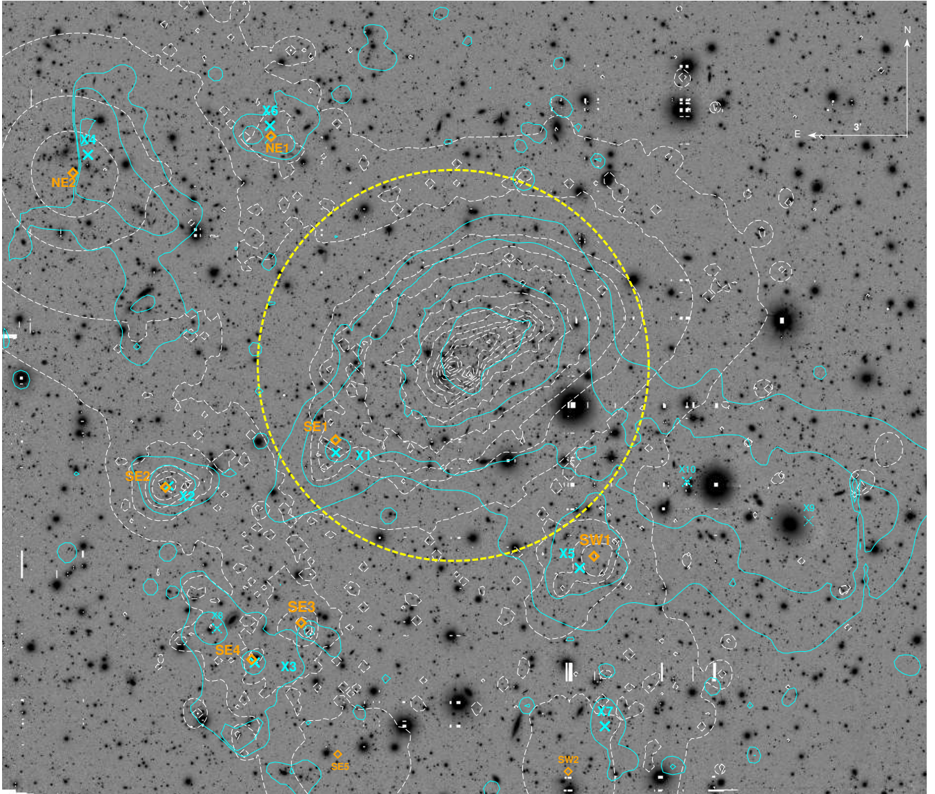
Figure 2. Subaru R-band image of MACSJ0717. Orange diamonds highlight the position of substructures detected in the strong+weak lensing mass map (and listed in Table 1); cyan crosses highlight the positions of remnant cores detected in the Chandra and XMM-Newton maps. White contours show the mass distribution derived from our strong+weak lensing mass model; cyan contours represent the gas distribution deduced from XMM-Newton observations. The yellow circle has a radius of R_{200} = 2.3 Mpc ( 5.8' ).
