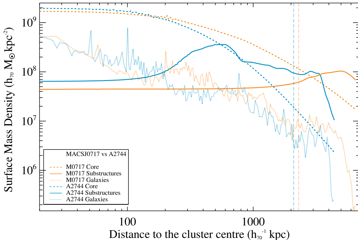
Figure 6. Density profile of the different components in MACSJ0717 (orange) and Abell 2744 (cyan) as a function of the distance to the cluster center: the core component (dashed line), the galaxy component (dotted lines) and the substructure component (plain lines). We differentiate between galaxies and (massive) substructures. The (long) dashed vertical lines highlight R_{200} for both clusters, MACSJ0717 and Abell 2744 in orange and cyan respectively.
