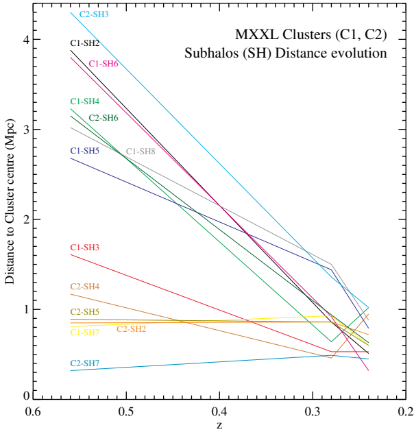
Figure 3. Projected distances to the main halo center as a function of redshift for the two MXXL clusters’ subhalos as listed in Table 4.
