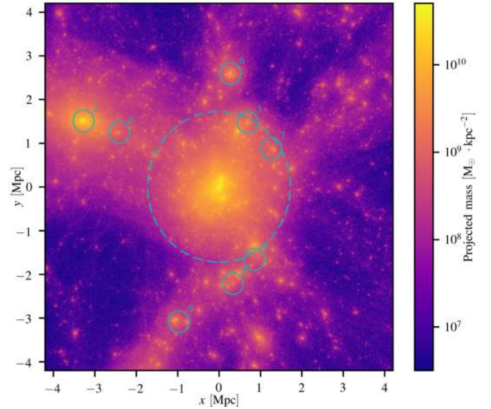
Figure 4. Projected mass map of halo CE-29 of the C-EAGLE simulation suite at z = 0.47 centered on the cluster’s minimum of potential. At this time the halo has a mass M_{200} = 9.15 \times 10^{14} M_{\odot} and a spherical overdensity radius R_{200} = 1.72 \text{ Mpc} (dashed circle). The small cyan circles indicate the eight subhalos that have a projected mass in a circular aperture of radius 250 kpc larger than our threshold for detection (see text for details). The overall distribution of sub-structures is in qualitative agreement with what is observed in the MACSJ0717 lensing mass map.
