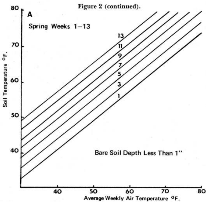
Figure 3. Nomographs for estimating soil temperature.
