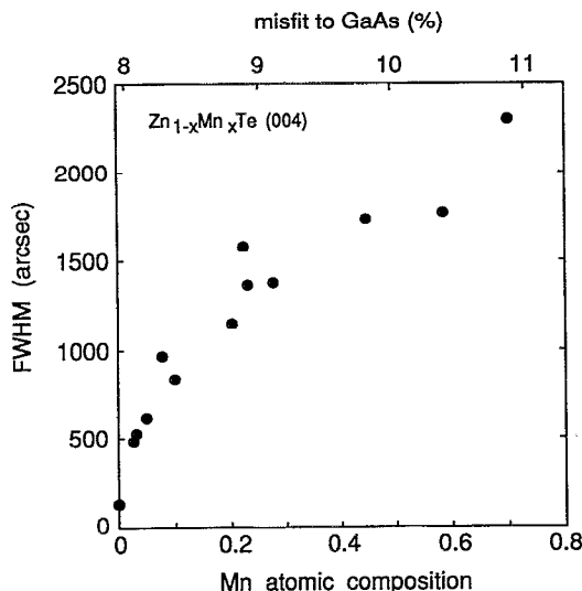
FIG. 3. FWHM of the (004) reflex of x-ray rocking curves as a function of the Mn content. The lattice misfit is also represented in this figure.
