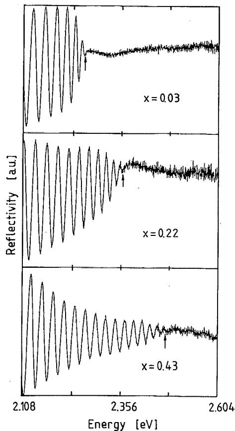
FIG. 1. Reflectivity spectra of three \text{Zn}_{1-x}\text{Mn}_x\text{Te} epilayers at 300 K. The arrows indicate the point where the interference fringes cease. This photon energy is used to determine the x values.
