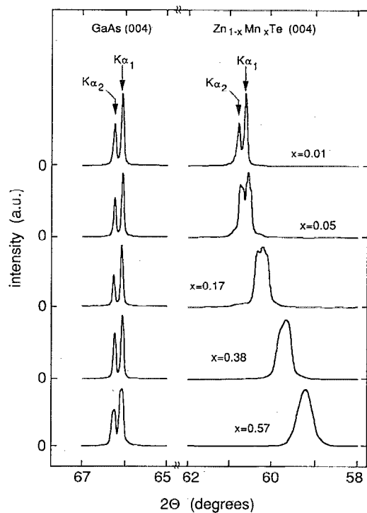
FIG. 2. \theta/2\theta scans of the (004) reflex of the \text{Zn}_{1-x}\text{Mn}_x\text{Te} epilayers and respective GaAs substrate.
