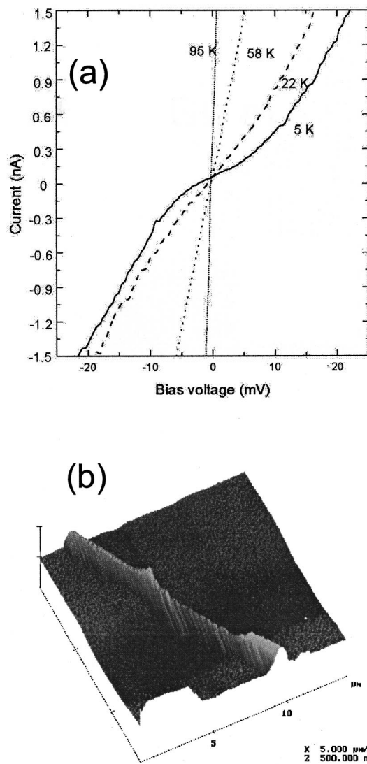
FIG. 5. (a) I - V curves of Ge nanowires at different temperatures, and (b) AFM image of a Ge nanowire device.
