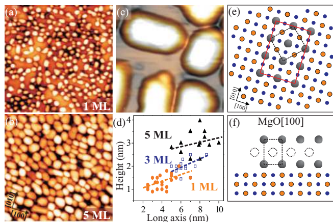
FIG. 3. (Color online) (a), (b) STM images of 10 ML MgO/Mo(001) taken after the indicated Ca exposure ( U_s = 5 V, 100 \times 100 nm 2 ). (c) Close-up image of a few Ca particles with characteristic shapes ( 10 \times 10 nm 2 ). (d) Statistical evaluation of the structural properties of Ca particles for different metal exposures. Structure model of a (001) plane of fcc Ca on the MgO surface: (e) top and (f) side view along the MgO[100] direction. The fcc Ca unit cell is marked by dashed lines; the particle edges are depicted by a red, solid rectangle. Filled and broken circles in (f) indicate atoms in the plane of view and the next plane, respectively.
