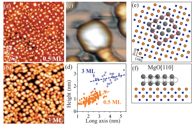
FIG. 6. (Color online) (a), (b) STM images of Fe particles on 10 ML MgO/Mo(001) ( U_s = 4.5 V, 100 \times 100 \text{ nm}^2 ). (c) Image of a characteristic Fe particle ( 10 \times 10 \text{ nm}^2 ). (d) Structural data of Fe deposits obtained for two different metal exposures. Structure model of the (001) plane of bcc Fe on the MgO surface: (e) top and (f) side view along the indicated crystallographic direction. All notations as in Fig. 3
