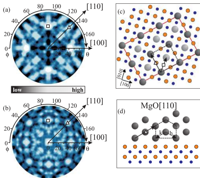
FIG. 2. (Color online) (a) Photoelectron diffraction (PED) stereogram of a Mg cluster film of 10 ML nominal thickness deposited on 10 ML MgO/Mo(001). The plot was taken at the Mg KLL Auger line at 1187 eV kinetic energy. (b) Simulation of the PED pattern using the MSCD package (Ref. 34). Main maxima are marked by squares and triangles in both plots and are explained in (c) and (d). Structure model of the (11\bar{2}0) hcp Mg plane that serves as interface to the oxide surface: (c) top and (d) side view along the MgO[110] direction. Mg atoms that need to be displaced to sit above an O atom are shown in gray. The Mg unit cell and the particle orientation are marked by a dashed square and a solid rectangle, respectively.
