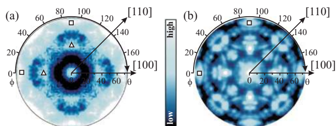
FIG. 5. (Color online) Experimental (a) and simulated (b) photoelectron diffraction stereogram of a Ni cluster film of 7 ML nominal thickness grown on 10 ML MgO/Mo(001). The data are taken at the Ni 2p core level ( E_{\text{kin}} = 1187 eV). The most prominent features are the four maxima along the MgO[100] direction that are indicated by the square.
