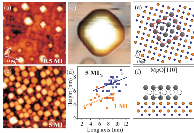
FIG. 7. (Color online) (a), (b) STM images of 10 ML MgO/Mo(001) for two different exposures of Ag ( U_s = 4.5 V, 100 \times 100 nm 2 ). For image (a), the sample has been slightly annealed to 550 K after Ag deposition. (c) Close-up image of a characteristic Ag particle ( 10 \times 10 nm 2 ). (d) Statistical evaluation of the geometry of Ag particles for two metal exposures. Structure model of the (001) plane of fcc Ag on the MgO surface: (e) top and (f) side view along the indicated crystallographic direction. All notations as in Fig. 3.
