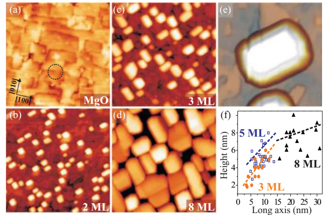
FIG. 1. (Color online) (a) STM image of a 10-ML-thick MgO film grown on Mo(001) ( 75 \times 75 nm 2 , U_s = 3.5 V). The dark lines are misfit dislocations that often emanate from screw cores (see circle). (b)–(d) Same film after deposition of increasing amounts of Mg ( 100 \times 100 nm 2 , U_s = 5 V). (e) Enlarged image of a characteristic Mg particle on the MgO surface ( 10 \times 10 nm 2 ). Note the identical orientation of the MgO film in all panels of this and the following figures. (f) Statistical evaluation of the heights and shapes of Mg particles for different metal exposures. Dashed lines are linear fits of the data, being used to deduce the aspect ratio of the deposits.
