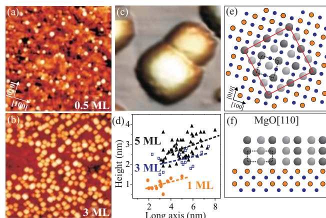
FIG. 4. (Color online) (a), (b) STM images of 10 ML MgO/Mo(001) for two different Ni exposures ( U_s = 3 V, 100 \times 100 nm 2 ). (c) Enlarged image of two characteristic Ni particles ( 10 \times 10 nm 2 ). (d) Statistical evaluation of the size and shape of Ni particles for different exposures. Structure model of the (11 \bar{2} 0) plane of hcp Ni on the MgO surface: (e) top and (f) side view along the indicated crystallographic direction. Other notations as in Fig. 2.
