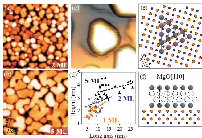
FIG. 8. (Color online) (a),(b) STM images of 10 ML MgO/Mo(001) after dosing with two different amounts of Au ( U_s = 5 V, 100 \times 100 nm 2 ). (c) Close-up image of a characteristic Au particle ( 10 \times 10 nm 2 ). (d) Statistical evaluation of the size and shape of Au particles for different exposures. Structure model of the (111) plane of fcc-Au on the MgO surface: (e) top and (f) side view along the indicated crystallographic direction. All notations as in Fig. 3.
