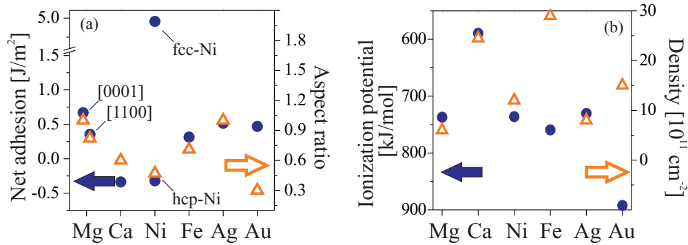
FIG. 9. (Color online) (a) Net adhesion (circles) between the indicated metal and an ideal MgO(001) surface, as calculated with the model described in the text. Apart from Au, the interfacial interaction correlates well with the mean aspect ratio of the deposits (triangles) as deduced from STM topographic images. (b) Comparison between the ionization potential (circles) and the particle density obtained after room temperature deposition of the indicated metals on MgO/Mo(001) (triangles). Again, the correlation is evident with the exception of gold and iron. See text for details.
