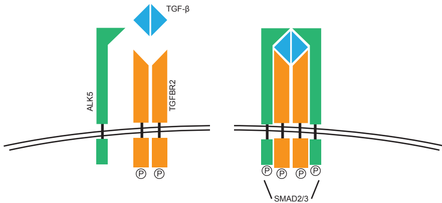
Figure 2. Assembly of the TGF- \beta /TGFBR2/ALK5 signaling complex.
