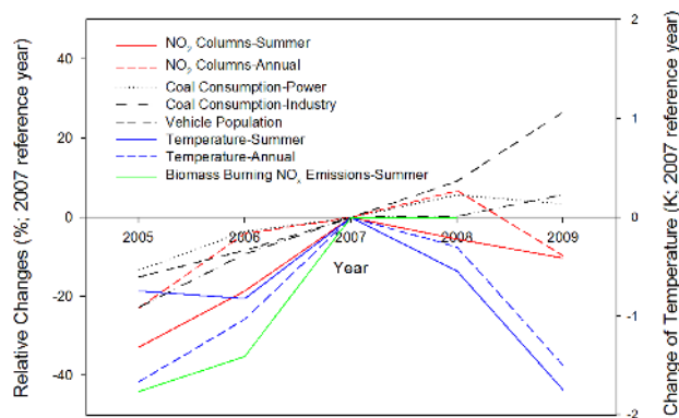
Fig. 9. Relative changes of annual and summer average OMI NO 2 columns, summertime biomass burning NO x emissions, and major anthropogenic activities, and absolute changes of annual and summer average temperature (2007 as reference year) during 2005–2009 in Northeast China. Summertime biomass burning emissions were taken from the GFED database (van der Werf et al., 2006).
