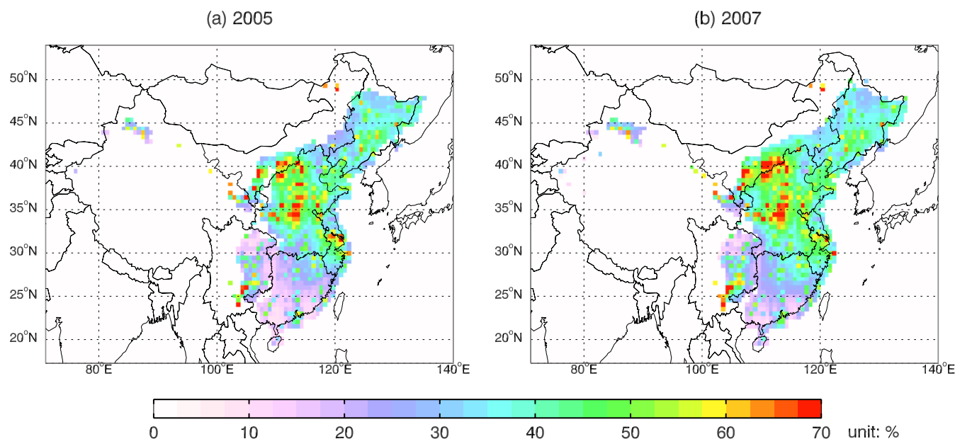
Fig. 11. Relative contributions of the power plant NO x emissions to the annual average NO 2 columns in (a) 2005 and (b) 2007, defined as the relative differences between GC_PP and GC_NoPP. Only grids inside Chinese boundary and with average NO 2 columns > 1.0 \times 10^{15} molecules cm -2 in GC_PP are colored.
