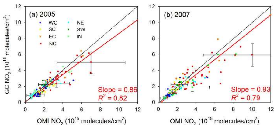
Fig. 3. Comparisons between GEOS-Chem and OMI summer average tropospheric NO 2 columns for (a) 2005 and (b) 2007 over power plant dominant grids in China. Grids are colored by the regions defined in Fig. 2. The linear fit regression (red line) is based on Reduced Major Axis (RMA) algorithm (Clarke, 1980). Error bars indicate the standard deviations in the summer average columns (only shown for minimum, quartiles, and maximum points in OMI datasets).
