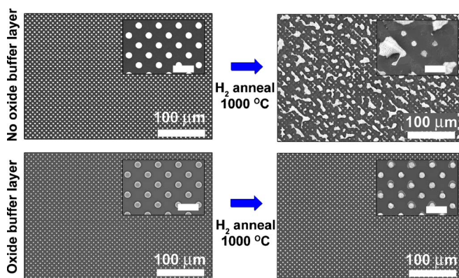
FIG. 1. (Color online) Effect of a 20 min anneal in \text{H}_2 , at 1000 \text{ }^\circ\text{C} and atmospheric pressure, on Au arrays with and without a 300 nm oxide buffer layer, demonstrating the importance of the buffer oxide in maintaining the pattern fidelity. The scale bars in the insets are 10 \mu\text{m} .
