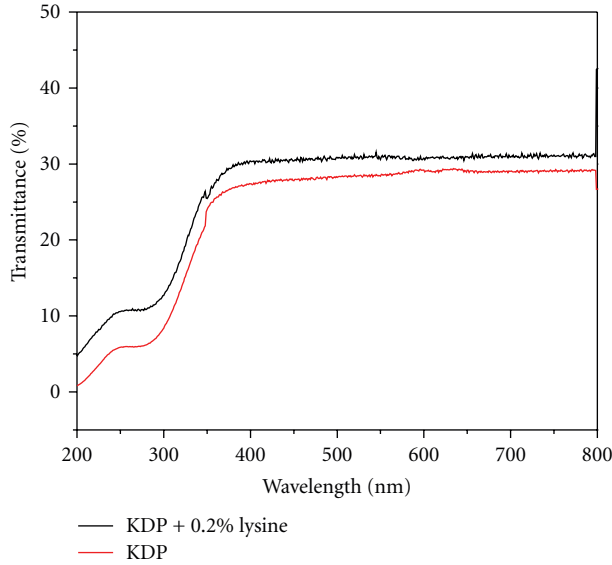
FIGURE 1: UV-Vis spectrum of pure and doped KDP crystals.
