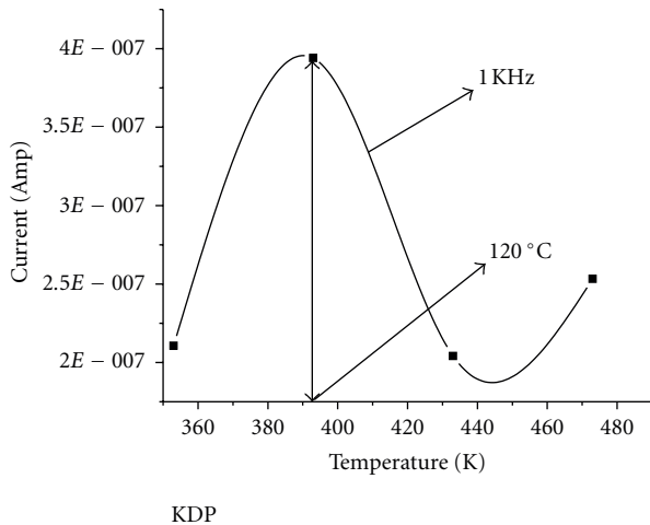
FIGURE 8: Variation in current with temperature.
