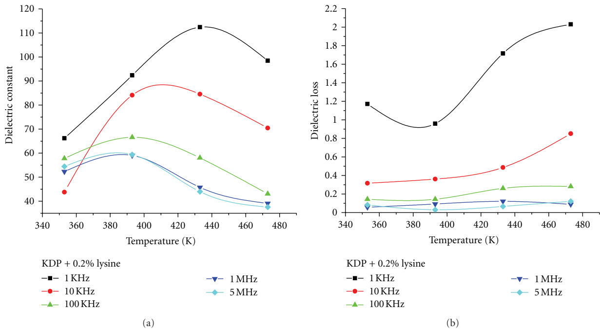
FIGURE 5: (a) variation of dielectric constant with temperature for all frequencies (lysine-doped KDP). (b) variation of dielectric loss with temperature for all frequencies (lysine-doped KDP).
