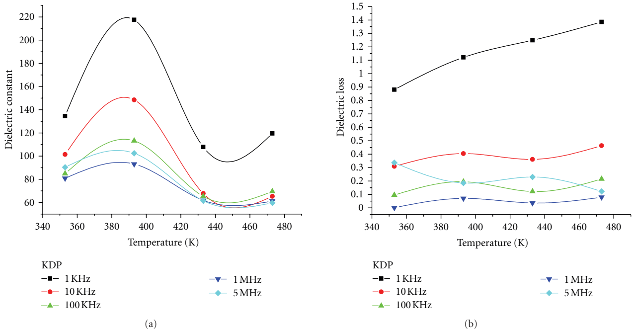
FIGURE 4: (a) Variation of dielectric constant with temperature for all frequencies (pure KDP). (b) Variation of dielectric loss with temperature for all frequencies (pure KDP).
