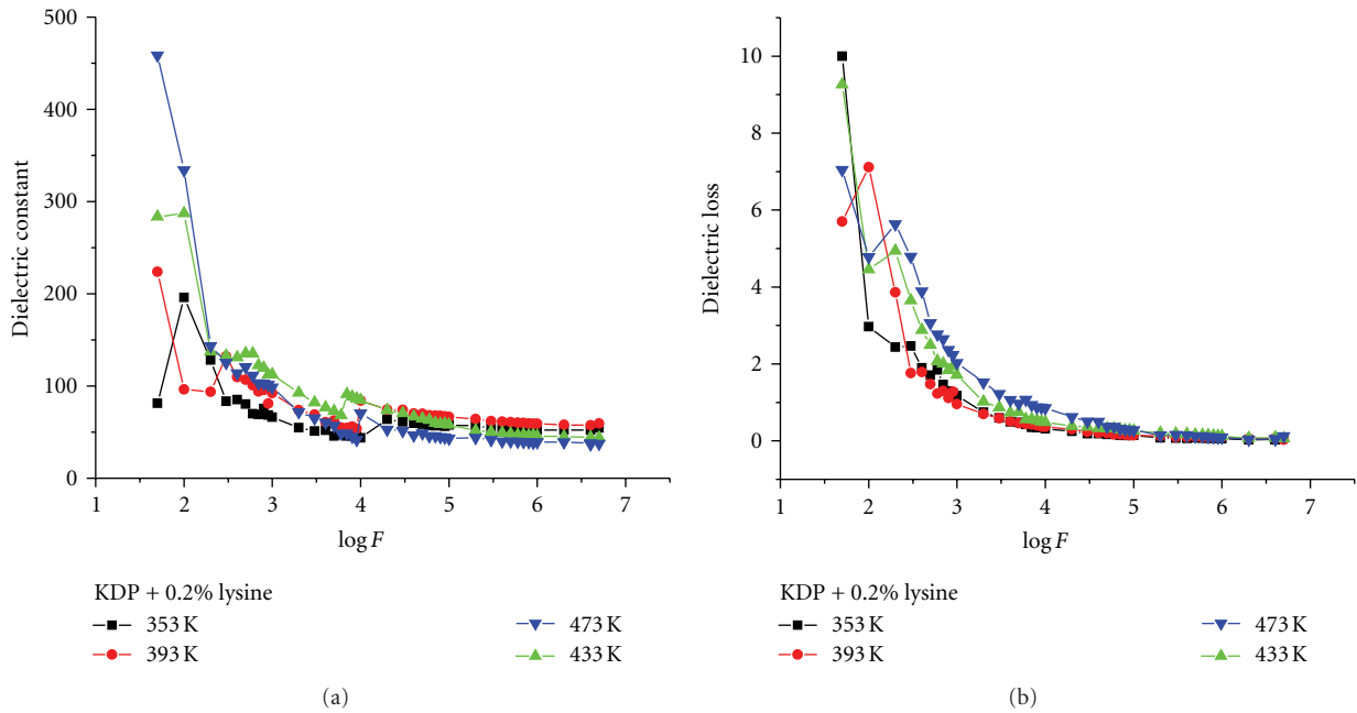
FIGURE 3: (a) variation of dielectric constant with frequency for all temperatures (lysine-doped KDP). (b) variation of dielectric loss with frequency for all temperatures (lysine-doped KDP).
