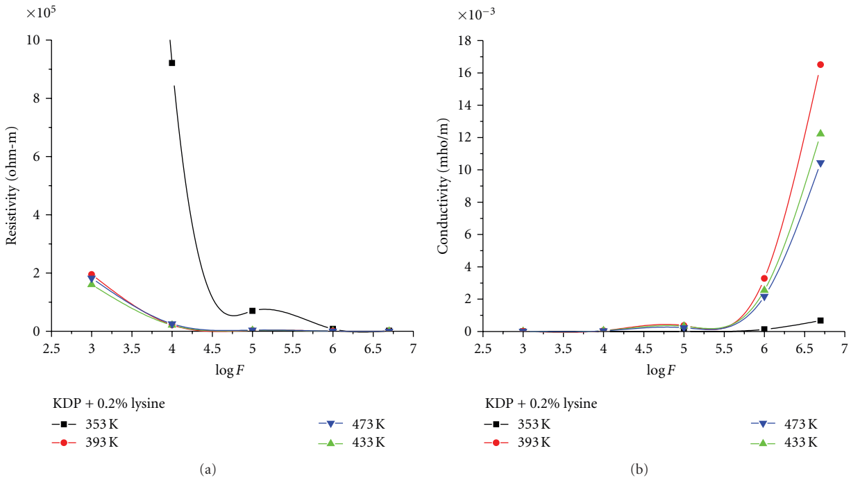
FIGURE 7: (a) Variation of resistivity with frequency (lysine-doped KDP). (b) Variation of conductivity with frequency (lysine-doped KDP).
