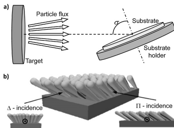
Figure 1. (a) Experimental setup; (b) definition of the \Delta and \Pi directions on the films.
