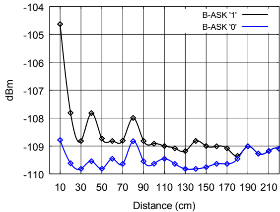
Figure 7: Signal strength received from WS1 (1600MHz, Dual) at various distances from the backside of the chassis.
