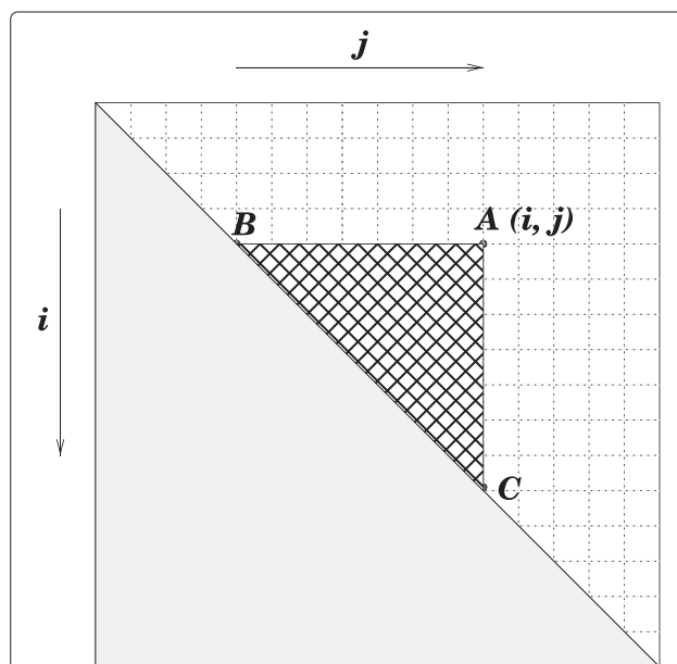
Figure 1 Dependencies. Figure 1 shows the dependencies in the dynamic programming algorithm. The (i, j) entry is dependent on the entries in the triangle (A, B, C) .
