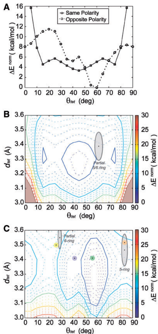
Figure 5. QM energy landscapes. (A) The rotational ( \theta_{tet} ) energy profile of same-polarity and opposite-polarity stacked G-tetrads at a d_{tet} value of 3.3 Å separation. Energy landscapes of (B) same-polarity and (C) opposite-polarity stacked tetrads are presented with stacking modes as determined from cataloged crystallographic structures superimposed. Average core G-tetrad stacking modes are shown with average geometries indicated by a black dot and gray outlined regions having dimensions of the first SD for \theta_{tet} and d_{tet} values. Average G-tetrad stacking modes at the interface of stacked G-quadruplexes are presented, color-coded as shown in Figure 4: ‘Partial 6-ring’ (yellow), ‘6-ring’ (purple), ‘5/6-ring’ (green) and ‘5-ring’ (orange).
