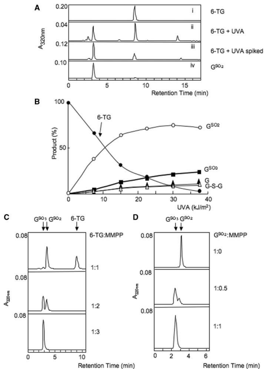
Figure 1. 6-TG/UVA photoproducts. (A) Identification of G^{\text{SO}_2} as a major photoproduct. 6-TG (0.1 mM in aqueous solution) was irradiated with 21 \text{ kJ/m}^2 UVA. Products were separated by HPLC System 1 as described in 'Experimental Procedures' section and the eluate monitored at 320 nm. (Top panel) Unirradiated 6-TG. (Second panel) 6-TG after 21 \text{ kJ/m}^2 UVA. (Third panel) As second panel, with authentic G^{\text{SO}_2} added before HPLC. (Bottom panel) Authentic G^{\text{SO}_2} (prepared by mild \text{I}_2 oxidation of 6-TG) alone. Unaltered 6-TG (filled circle) eluted at 9 min. Quantitation was at the absorbance maximum for each product and by comparison to authentic standard compounds. G^{\text{SO}_3} ( A_{325} ), G^{\text{SO}_2} ( A_{320} ), G ( A_{273} ), 6-TG ( A_{340} ) and G-S-G ( A_{331} ). Products are expressed mole % of unirradiated 6-TG. A representative of three independent experiments is shown. (C) 6-TG oxidation by MMPP. 6-TG (0.1 mM) was treated for 10 min at 20^\circ\text{C} with MMPP at the final molar ratio indicated. Products were separated by HPLC System 2 and eluates monitored at 320 nm. Unchanged 6-TG elutes at 9 min, G^{\text{SO}_2} at 3.5 min and G^{\text{SO}_3} at 3.0 min. (D) G^{\text{SO}_2} oxidation by MMPP. G^{\text{SO}_2} (0.1 mM) was treated for 10 min at 20^\circ\text{C} with MMPP at the molar ratios shown. Products were separated by HPLC System 3.
