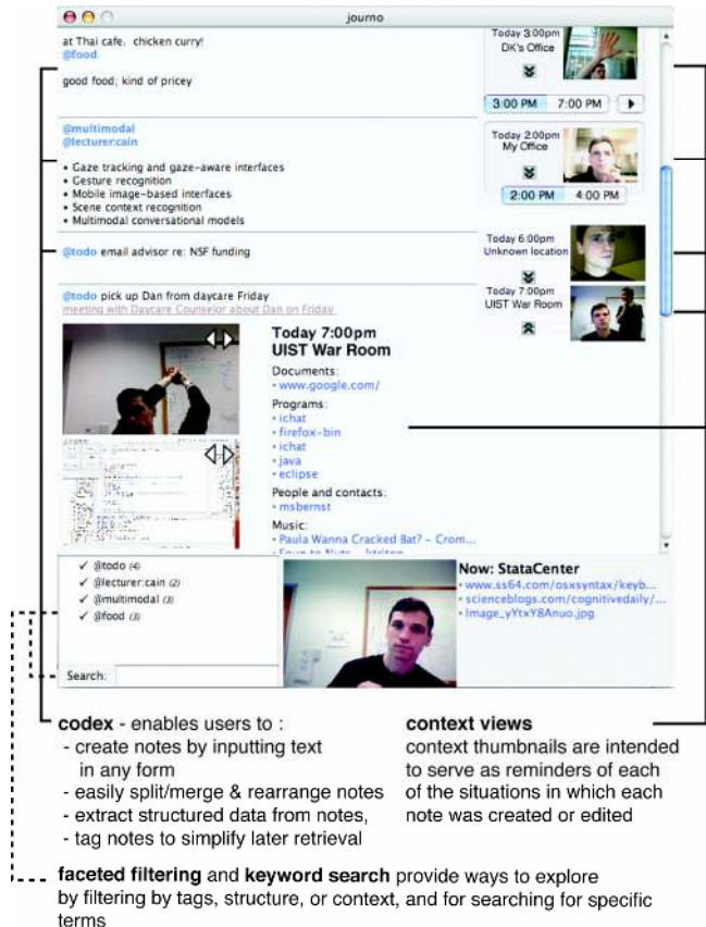
Figure 1: The Jourknow interface displaying the set of textual notes, which we collectively refer to as the codex . In addition to the text, Jourknow's side panels provide facilities for quickly scanning notes through episode thumbnails and navigating non-linearly by filtering notes according to facets that characterize their contents. The current context display (bottom right) provides a preview of how the current editing session will be later portrayed in epi-
