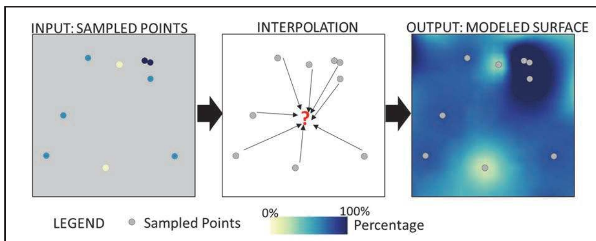
Figure 1. Interpolation process
