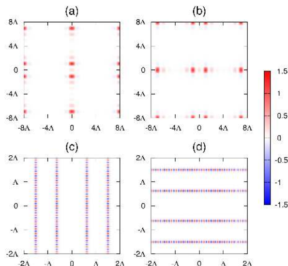
Fig. 7. Two examples of pairs of non-symmetric modes. (a) and (b) Air-guided modes generated by the symmetric modes shown in Figs. 4(a) and 4(e). (c) and (d) Glass-guided modes formed by the combination of the high-index mode of Fig. 5(b) and the delocalised mode of Fig. 6(a). The (\beta\Lambda)^2 values are 1579.93 for modes (a) and (b), and 2073.28 for modes (c) and (d).
