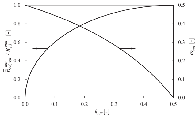
Figure 6. Effect of the microstructure of the composite electrode on the optimal conditions of mesoscale structural modification according to Eq. 13 in the limit t_{ed} = t_h \rightarrow \infty . Ratio between optimal electrode resistance and minimum resistance of flat electrode (left axis) and optimal volume fraction of pillars (right axis) as a function of the effective conductivity factor of the composite electrode domain.
