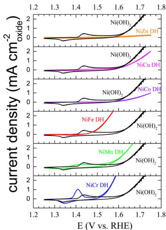
Figure 5. Cyclic voltammetry for the OER in 0.1 M KOH of nickel-based DH immobilized on Au. Experiments were performed under hydrodynamic conditions ( \omega = 1500 rpm, \nu = 0.01 V s -1 ). The black line shows the activity of Ni(OH) 2 , presented as a benchmark of the catalytic activity.
