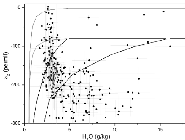
Fig. 9. \delta_D (‰) as a function of \text{H}_2^{16}\text{O} (g/kg) for the 8 October 2007 during Krosa typhoon overpass in South-East Asia. The full black circles show the morning data averaged on a 1^\circ \times 1^\circ longitude-latitude grid and the light grey crosses are their uncertainties associated. The black lines represent the Rayleigh distillation curves with surface temperatures of 288 K (left line) and 300 K (right line), initialized to the surface layer \delta_D value of -79 ‰. The grey lines represent evaporation lines initialized respectively from the same value of \delta_D ( -79 ‰) (lower grey line) and the average seasonal \delta_D value in regional precipitation (based on Global Network of Isotopes in Precipitation (GNIP) observation).
