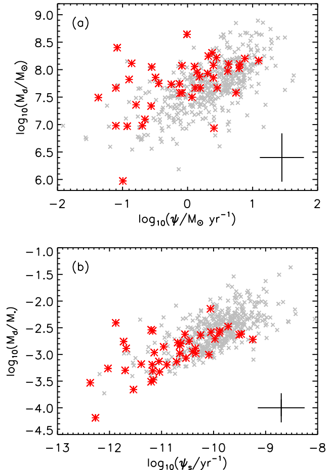
Figure 6. (a): M_d vs. SFR of the ETGs (large red stars) compared to the spiral galaxies (small grey crosses). (b): M_d/M_* vs. SSFR of the ETGs compared to the spiral galaxies. The error bars indicate the median 1\sigma uncertainty on a data point.
