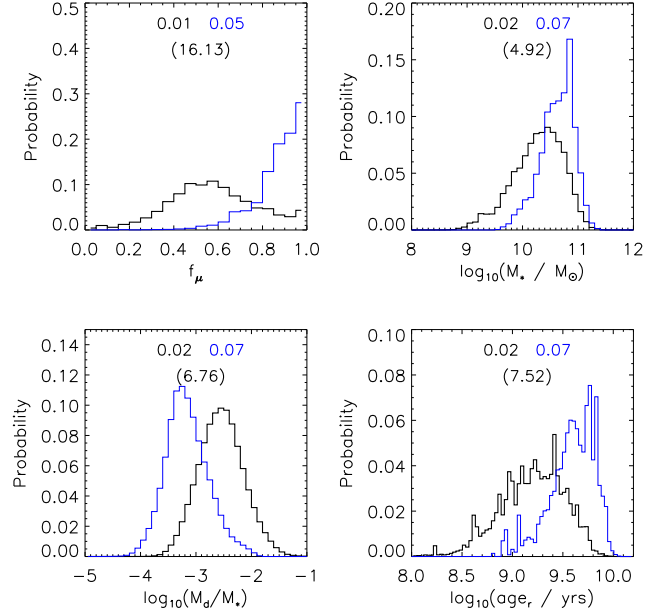
Figure 9. Average PDFs of the SED parameters of 19 passive spirals ( SSFR < 10^{-11} \text{yr}^{-1} ) (blue line) compared to 431 normal spirals with SSFR \geq 10^{-11} \text{yr}^{-1} (black line). The parameters are (from left to right): f_\mu , the fraction of total dust luminosity contributed by the diffuse ISM; M_* , stellar mass; M_d/M_* , dust to stellar mass ratio; and age_r , the r -band light-weighted age of the stellar population. The uncertainty on each distribution for ETGs and spirals is given by the error on the mean and is shown at the top of each histogram with corresponding colours, and the significance of the difference in the means in brackets. The errors for logarithmic parameters are in dex.
