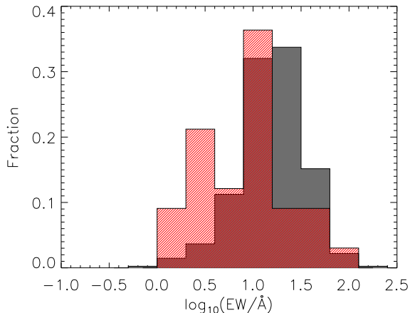
Figure 11. H\alpha EW (corrected for stellar absorption) of spiral galaxies (grey) and ETGs (red/hatched) which have \geq 3\sigma H\alpha detections. A K-S test shows that the ETGs have a probability of 1.7 \times 10^{-4} of being drawn from the same distribution as the spirals.
