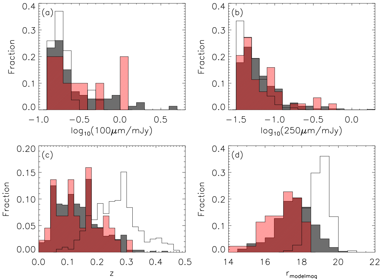
Figure 1. The distribution of \geq 5\sigma 100\mu\text{m} (a) and 250\mu\text{m} point-source fluxes (b) are shown for the H-ATLAS morphologically classified sample. Spirals are shown as grey-filled, ETGs as red/hatched and unknown morphologies as an open histogram. It can be seen that the flux distributions are similar for each type of morphology. (c): Redshift distribution of our H-ATLAS sample for each morphological type. The ETGs and spirals have similar redshift distributions, but galaxies classified as unknown lie at much higher redshift on average. (d): The distribution of SDSS r -band model magnitudes for the same morphological classifications. Sources with unknown morphologies are fainter on average than those which are classified.
