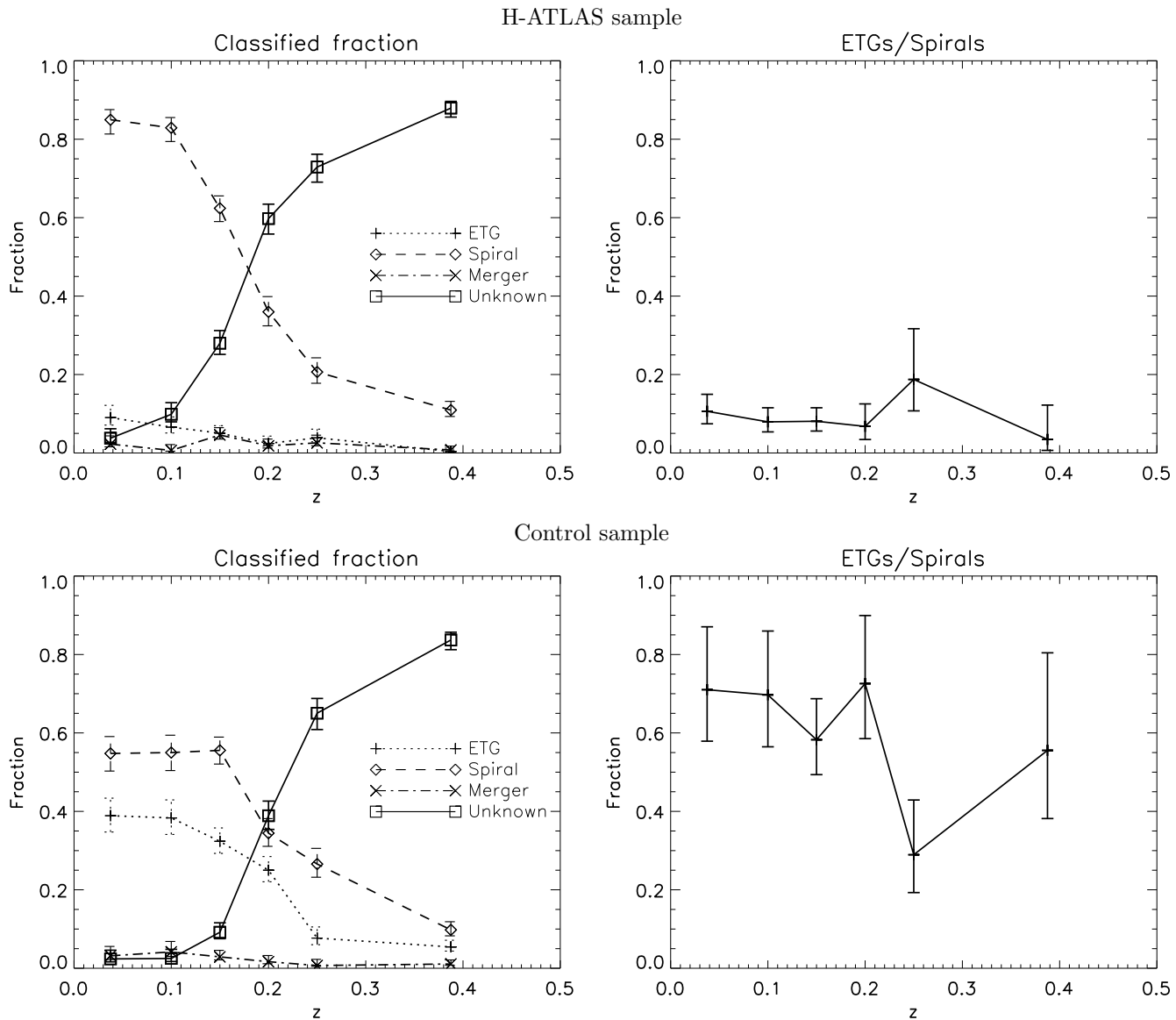
Figure 3. Morphological classification fractions as a function of redshift for the H-ATLAS detected sample (top) and the control sample (bottom). Errors bars are the 1\sigma confidence intervals for a binomial population, derived from a beta distribution (see Cameron 2011). Also shown is the ETG-to-spiral fraction for both samples, where error bars are the 1\sigma confidence intervals for a binomial distribution, using the approximation of Gehrels (1986). The ETG-to-spiral fraction does not increase with redshift, therefore we do not observe a bias towards classifying more ETGs as they become smaller and fainter.
