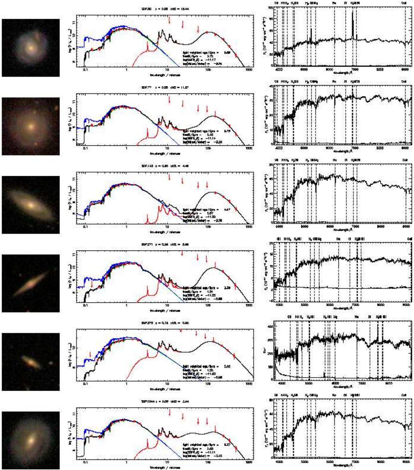
Figure B1. Optical images, multiwavelength SEDs and optical spectra of the 19 passive spirals in our sample. Images are 40'' on a side. The rest-frame SEDs of each passive spiral are shown, where red points are the observed photometry, with 5\sigma upper limits shown as arrows. Errors on the photometry are described in Smith et al. (2011b). The black line is the total best fit SED model, the green line is the attenuated optical model, the blue line is the unattenuated optical model, the red line is the infrared model. Spectra are from SDSS and GAMA, and the standard deviation in the spectra is also shown. The spectra have been smoothed by a boxcar of 8 pixels.
