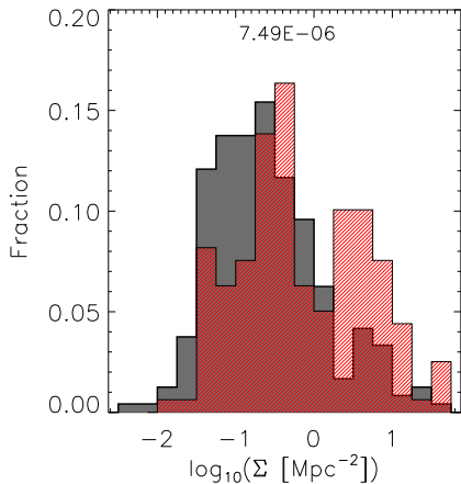
Figure 16. Comparison of densities for control sample ETGs (red/hatched) and spirals (grey). As expected, the spirals have a lower median density than the ETGs. A K-S test shows a low probability of the samples of ETGs and spirals being drawn from the same distribution.
