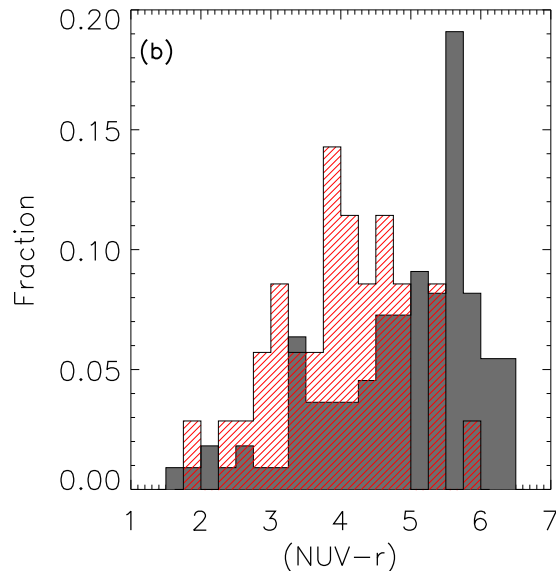
Figure 15. (a): UV-optical colour magnitude diagram for H-ATLAS detected (red stars) and control ETGs (grey crosses). Lower limits are shown for galaxies which do not have a \geq 5\sigma NUV detection. (b): Comparison of the NUV-r colours for the detected ETGs (red/hatched) and control ETGs (grey/filled)
