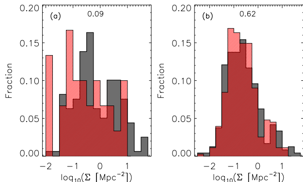
Figure 17. Comparison of environments between H-ATLAS detected (red/hatched) and control ETGs (a) and H-ATLAS and control spirals (b). For the detected and control ETGs a K-S test shows the two distributions have a low probability of being drawn from the same distribution, although this is only significant at the 1.8\sigma level. We cannot statistically rule out the null hypothesis that the control and H-ATLAS spirals are drawn from the same distribution.
