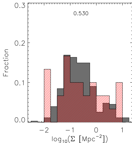
Figure 12. Comparison of densities for H-ATLAS spirals (grey) and ETGs (red/hatched). A K-S test (shown at top of histogram) shows that we can’t statistically rule out the null hypothesis of the samples being drawn from the same distribution.
