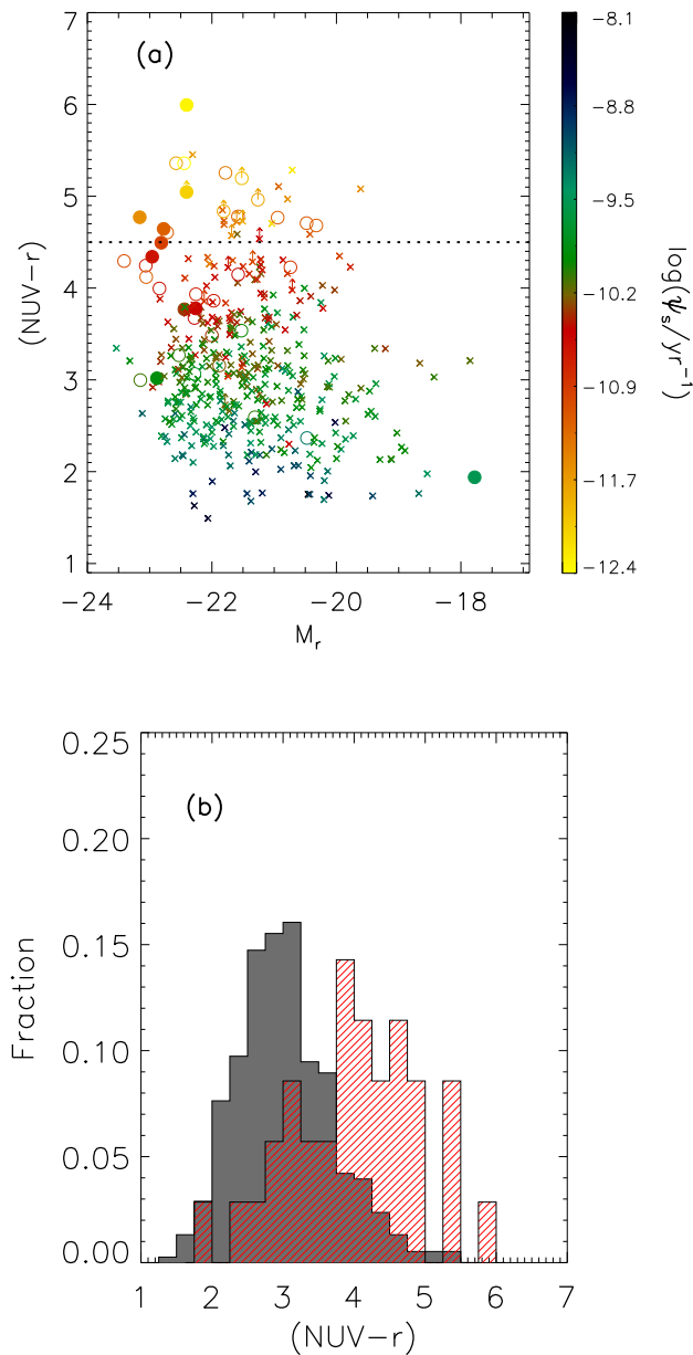
Figure 8. (a): UV-optical colour magnitude diagram, colour coded according to SSFR. Circles are ETGs, crosses are spirals, filled circles indicate that the ETG is morphologically disturbed. The dashed line shows the separation between ‘blue’ and ‘red’ as defined in Dariush et al. (2011). Lower limits are shown for galaxies which do not have a \geq 5\sigma NUV detection. (b): The distribution of (NUV - r) colours for the ETGs (red/hatched) and spirals (grey) which have a \geq 5\sigma NUV detection.
