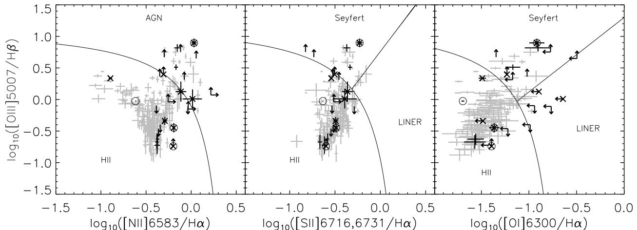
Figure 10. BPT diagram showing H-ATLAS spirals (grey) and ETGs (black) with all four lines in each diagram detected at > 3\sigma , with error bars shown. Those below the curved line are classified as star-forming, those above the curved line are classified as AGN. Upper limits are shown for the ETGs where at least two emission lines are detected. ETGs which have radio emission (Section 5.3) are marked with a circle, and disturbed morphologies with a diagonal cross.
