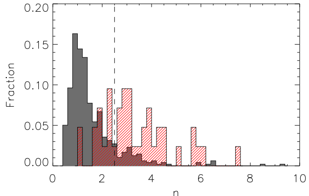
Figure 2. Sérsic index ( n ) distribution of the spirals (grey), and ETGs (red/hatched) in our H-ATLAS sample. The dashed line at n = 2.5 denotes the traditional cut between ‘early-type’ ( n > 2.5 ) and ‘late-type’ ( n < 2.5 ), and gives an indication of the contamination that can occur in samples selected on Sérsic index.
