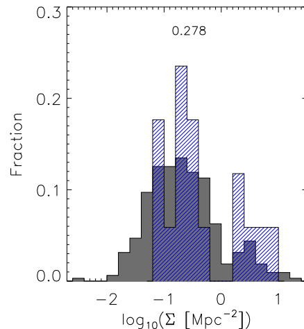
Figure 13. Environment of passive spirals with \text{SSFR} < 10^{-11}\text{yr}^{-1} detected in H-ATLAS (blue), compared to normal spirals with \text{SSFR} > 10^{-11}\text{yr}^{-1} (grey). A K-S test shows a high probability (shown at top of histogram) that both samples are drawn from the same distribution.
