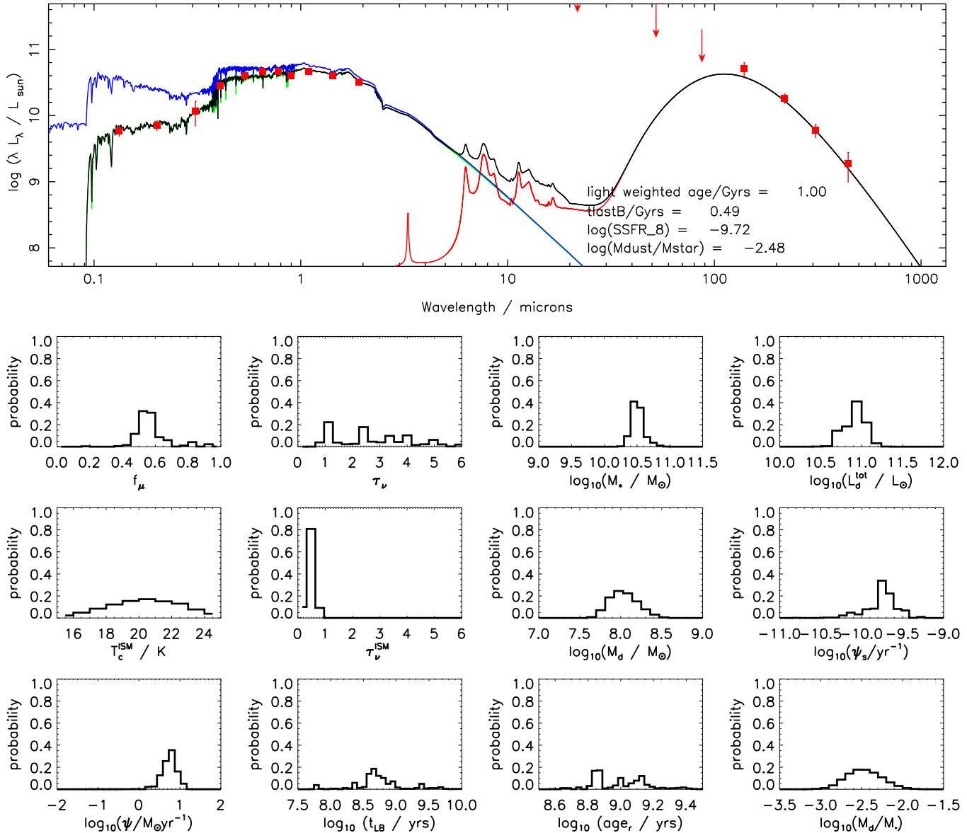
Figure 4. Top: Example best-fit rest-frame SED of an ETG, with observed photometry points from the UV to the submillimetre (red squares). 5\sigma upper limits are shown as arrows. Errors on the photometry are described in Smith et al. (2011b). The black line is the best fit model, the green line is the attenuated optical model, the blue line is the unattenuated optical model, and the red line is the infrared model. Bottom: probability density functions of parameters for this ETG.
