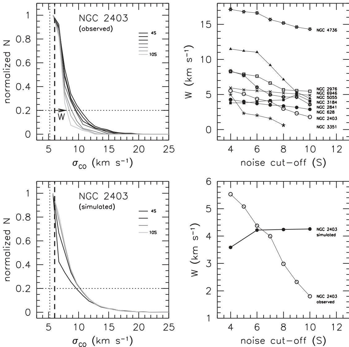
Figure 8. Top left: normalized distributions of \sigma_{\text{CO}} for NGC 2403 for different values of the noise cutoff. The black curve indicates a 4S cutoff. From black to light gray, the noise cutoff increases in steps of S with the light-gray curve indicating a 10S cutoff. It is clear that the curves become narrower with increasing noise cutoff. The thick dashed vertical line indicates the mode of the distribution, the dotted vertical line the velocity resolution cutoff. The horizontal dotted line indicates the 20% level at which the width with respect to the mode is measured. The width W is indicated for the 10S curve by the arrow labeled “ W .” Bottom left: normalized distributions of the simulated NGC 2403 data for different peak-flux values. Velocity profiles were simulated with random noise, varying input amplitudes, and input dispersions drawn from NGC 2403’s 4S\sigma_{\text{CO}} distribution. The profiles were fitted in the same manner as the observed data and the histograms of the fitted dispersions are plotted. Top right: the 20% width W as defined in the left panel plotted against the noise cutoff in units of S . Galaxies are labeled to the right of their corresponding curve. Note that for NGC 3351 only values up to 8S could be measured. Bottom right: the W values of the observed NGC 2403 \sigma_{\text{CO}} distributions and the simulated distributions are plotted against the modeled peak-flux value.
