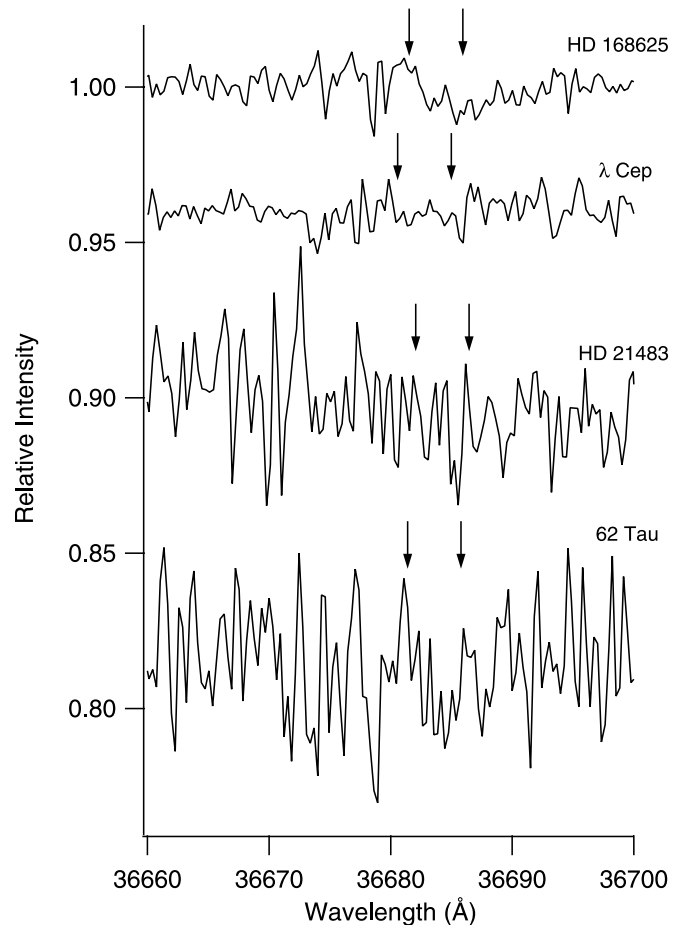
FIG. 5.—Same as Fig. 2, but showing nondetections.
