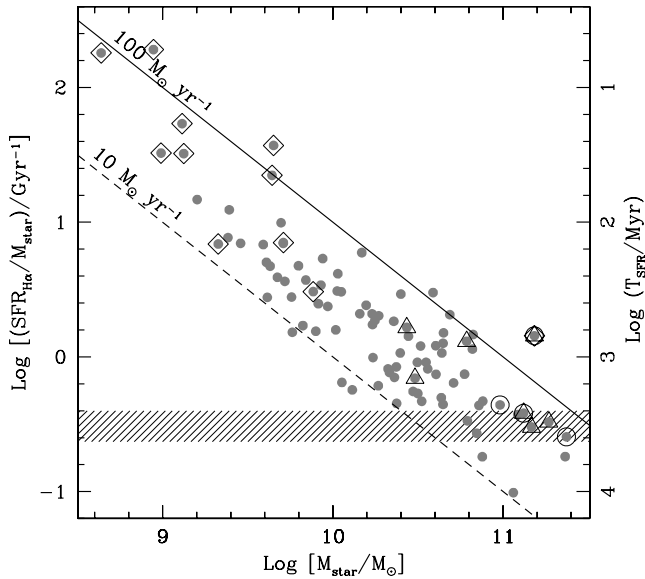
FIG. 5.—Specific star formation rate \text{SFR}_{\text{H}\alpha}/M_* vs. stellar mass. The solid and dashed diagonal lines show SFRs of 100 and 10 M_{\odot} \text{ yr}^{-1} , respectively. The right axis shows the SFR timescale T_{\text{SFR}} = M_*/\text{SFR}_{\text{H}\alpha} , the inverse of the specific SFR. On this scale, the shaded band represents the age of the universe for the redshift range of the galaxies in the sample. The most massive galaxies have T_{\text{SFR}} \gtrsim t_{\text{universe}} , indicating that they may require declining star formation histories. Symbols are as in Fig. 4. [See the electronic edition of the Journal for a color version of this figure.]
