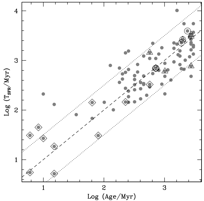
FIG. 6.—Star formation timescale T_{\text{SFR}} vs. age. This plot provides a check of the consistency of the \text{H}\alpha SFRs and the primarily constant star formation models we use to fit the SEDs; for CSF models, T_{\text{SFR}} should be approximately equal to the age. The dashed line shows equal times, and the dotted lines on either side show the typical uncertainty in age. Symbols are as in Fig. 4. [See the electronic edition of the Journal for a color version of this figure.]
