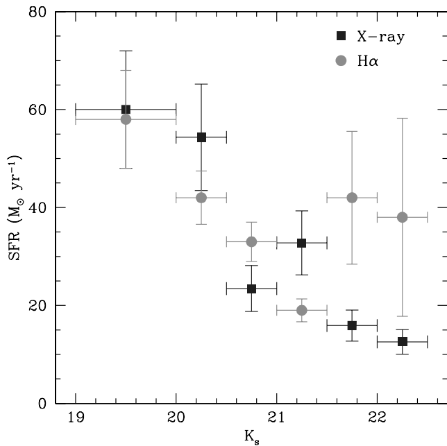
FIG. 2.—SFRs from H \alpha and X-ray stacking, as a function of K magnitude. Circles from left to right represent the average extinction-corrected SFR _{\text{H}\alpha} of galaxies with 19 < K_s \leq 20 and in 0.5 mag bins between K_s = 20 and 22.5, excluding AGNs. The average SFRs determined by stacking deep X-ray images of a slightly overlapping sample of z \sim 2 galaxies in the GOODS-N field in the same ranges of K magnitude are shown by the squares (Reddy et al. 2005). The upturn in SFR _{\text{H}\alpha} at faint K magnitudes is probably a selection effect, because we are less likely to detect H \alpha in galaxies faint in K and because X-rays may underestimate the SFRs for young objects. [See the electronic edition of the Journal for a color version of this figure.]
