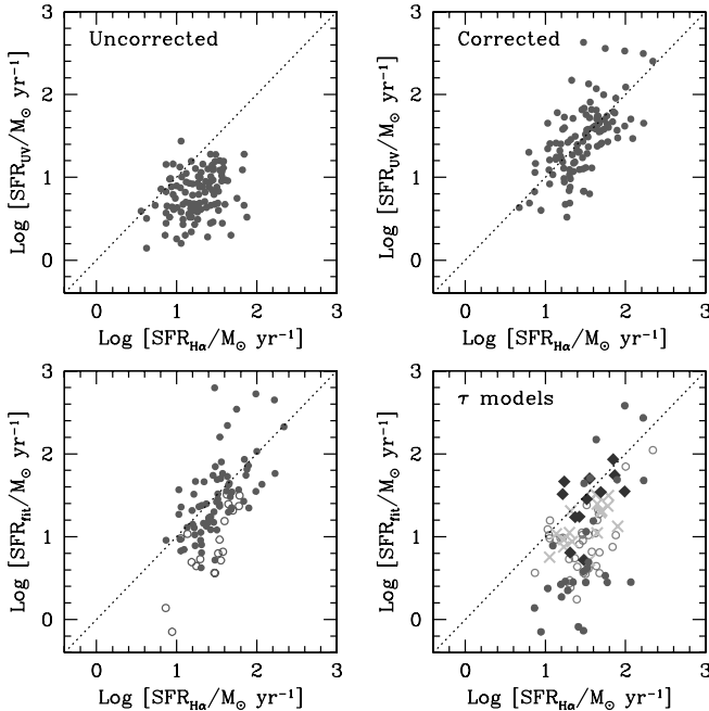
FIG. 1.—Comparison of star formation rates from H \alpha , the UV continuum, and the SED fits. Top left : SFR _{\text{H}\alpha} vs. SFR _{\text{UV}} , without correcting for extinction. Top right : SFR _{\text{H}\alpha} vs. SFR _{\text{UV}} , with both SFRs corrected for extinction. Bottom left : Corrected SFR _{\text{H}\alpha} vs. the SFR obtained from the normalization of the adopted model SED. Solid symbols are constant star formation models, and the open symbols represent objects for which we have adopted a model with an exponentially decreasing star formation rate. Bottom right : Corrected SFR _{\text{H}\alpha} vs. the SFR of the best-fitting declining model for each object. Filled circles are galaxies with \tau = 10, 20, \text{ or } 50 Myr, open circles have \tau = 100, 200, \text{ or } 500 Myr, crosses have \tau = 1, 2, \text{ or } 5 Gyr, and diamonds are constant star formation models. The use of steeply declining \tau models decreases the SFR with respect to that found from H \alpha . [See the electronic edition of the Journal for a color version of this figure.]
