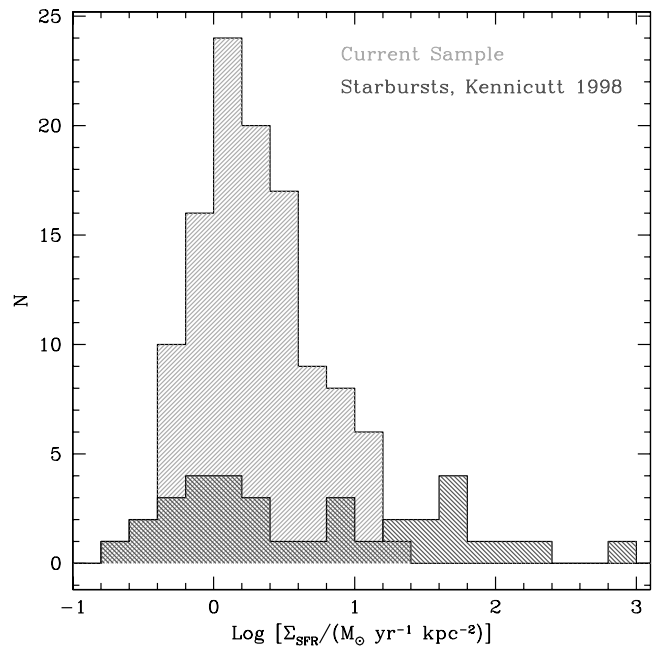
FIG. 3.—Comparison of the star formation surface densities \Sigma_{\text{SFR}} of the current sample ( large histogram ) and the starbursts of Kennicutt (1998b, short histogram ). In this case we use a Salpeter IMF for consistency with the low-redshift sample. The inability to resolve star formation on small spatial scales at high redshift results in an absence of objects with the highest values of \Sigma_{\text{SFR}} in the z \sim 2 sample. [See the electronic edition of the Journal for a color version of this figure.]
