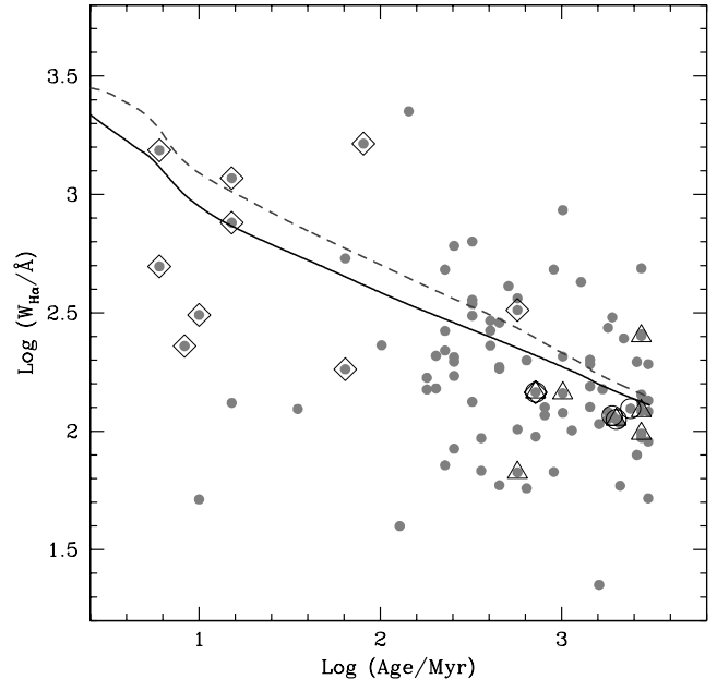
FIG. 7.—Comparison of H\alpha equivalent width and age from the SED modeling. The lines show the predicted W_{H\alpha} as a function of age for constant star formation, from Starburst99 models with solar (solid line) and 0.4 solar (dashed line) metallicity. The large scatter of the data with respect to the models is probably caused by variations in the SFR as well as observational uncertainties. Symbols are as in Fig. 4. [See the electronic edition of the Journal for a color version of this figure.]
