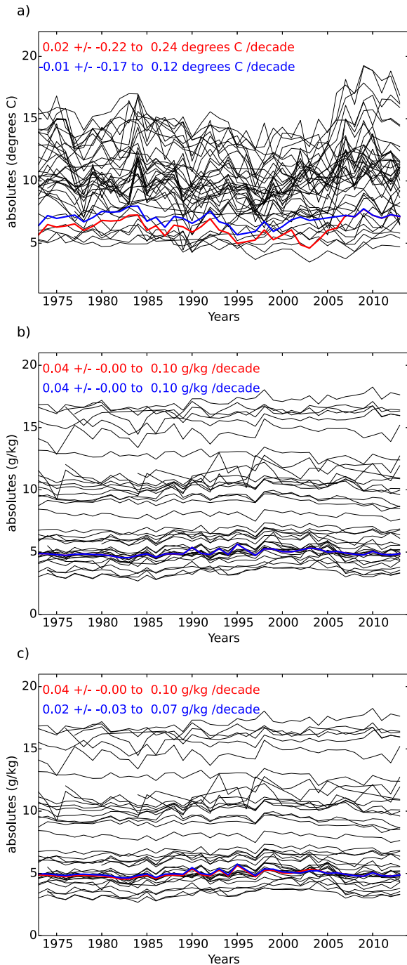
Figure 4. Example of an inhomogeneity having a greater signal-to-noise ratio in DPD compared to q for station 557 730, Pagri, Tibet. (a) DPD annual mean series for raw data (red) and direct PHA homogenised data (blue) for 557 730 and its raw neighbour series (black). (b) q annual mean series for raw data (red) and direct PHA homogenised data (blue) for 557 730 and its raw neighbour series (black). (c) q annual mean series for raw data (red) and indirect PHA homogenised data (blue) for 557 730 and its raw neighbour series (black).
