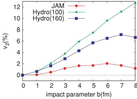
FIG. 3. (Color online) Elliptic flow v_2 for charged hadrons at midrapidity as a function of impact parameter in Cu+Cu collisions at \sqrt{s_{NN}} = 200 GeV. Circles connected by line show the results of JAM. Triangles and squares with lines show the results of hydrodynamics with T^{\text{th}} = 100 MeV and 160 MeV, respectively.
