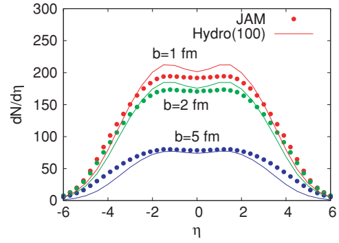
FIG. 1. (Color online) Pseudorapidity distributions for charged hadrons in Cu+Cu collisions at \sqrt{s_{NN}} = 200 GeV for impact parameters b = 1, 2, and 5 fm. Circles correspond to the result of JAM. Lines denote the results of hydrodynamics for T^{\text{th}} = 100 MeV.
