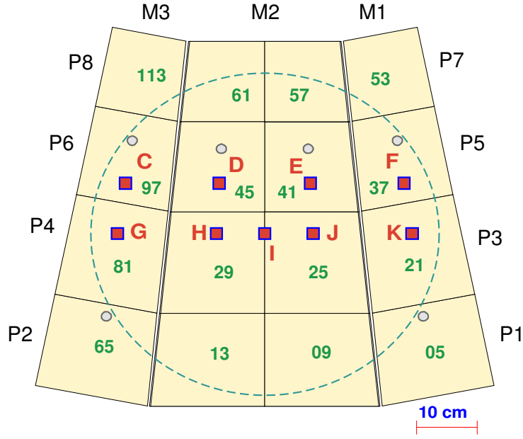
Fig. 8. Position of the beam impact points (C-K) on the front face of HEC1. The large circle indicates the beam window; the small circles the position of the tie rods
