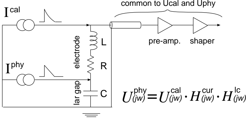
Fig. 6. Schematic EMEC read-out chain and calibration network. The variables U^{\text{phy}}(j\omega) and U^{\text{cal}}(j\omega) are the pulse shapes in the frequency domain for the physics and calibration pulses, respectively.
