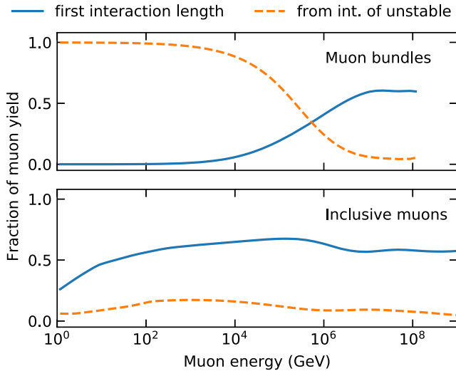
FIG. 8. Red dashed lines show the contribution to the muon spectrum by interactions of unstable particles ( \pi^\pm , \Lambda , etc.) and solid blue the fraction of muons that is related to hadronic interactions in the first interaction length ( \sim 90 g/cm ^2 ) of the cosmic ray nucleon. The upper panel is computed for a single 100 PeV proton and a vertical incidence angle.
