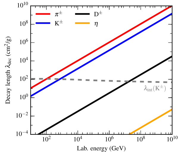
FIG. 1. Decay lengths for relevant mesons (solid) compared to the interaction length for kaons calculated at 8 km altitude a.s.l.
