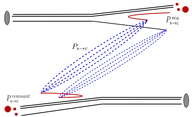
FIG. 19. String configuration with remnant excitation. Note that the flavor content of the remnant can be different from the initial hadron in the case of remnant excitation.
