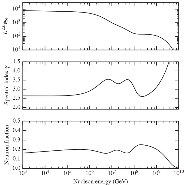
FIG. 2. Upper panel: Flux of nucleons in (\text{m}^2 \text{sr GeV}^{1.6})^{-1} , converted from the flux of cosmic ray nuclei as predicted by the H3a model. Middle panel: spectral index, log-derivative of the upper curve. Lower panel: Fraction of neutrons in the nucleon flux. The spectral softening at around 1 PeV is an effect of the knee and the hardening at \sim 100 PeV of the ankle of cosmic rays.
