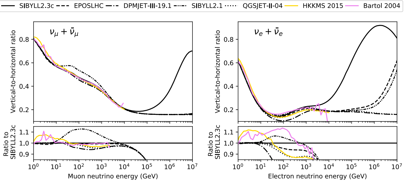
FIG. 38. Down to horizontal ratio. It is defined as the ratio of fluxes integrated in the angular bin \cos \theta < 0.4 around the two extreme directions. The comparison is shown down to the lowest energies, since it is strongly impacted by 3D calculations at energies below a few GeV. Large differences at high energy originate from the presence of prompt neutrinos in the SIBYLL-2.3c calculations.
