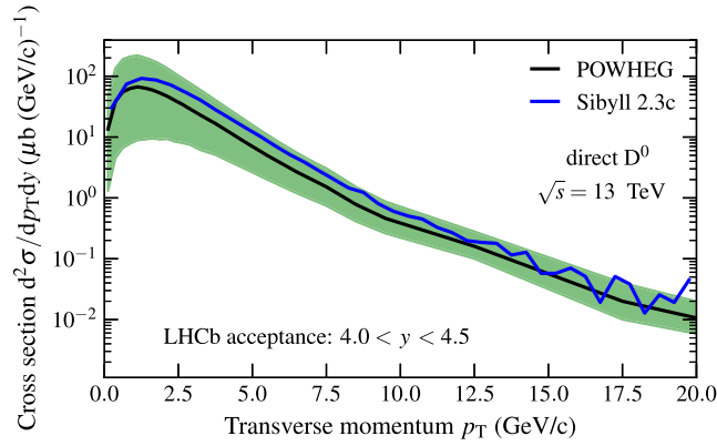
FIG. 25. p_T -spectrum of neutral D-mesons at \sqrt{s} = 13 TeV. Compared are SIBYLL and a NLO QCD calculation (POWHEG) [65]. The band of the theory calculation corresponds to charm quark mass and factorization scale uncertainty. The central phase space covered by the LHCb acceptance is dominated by perturbative processes, such that the full prediction by SIBYLL can be compared to the pQCD calculation.
