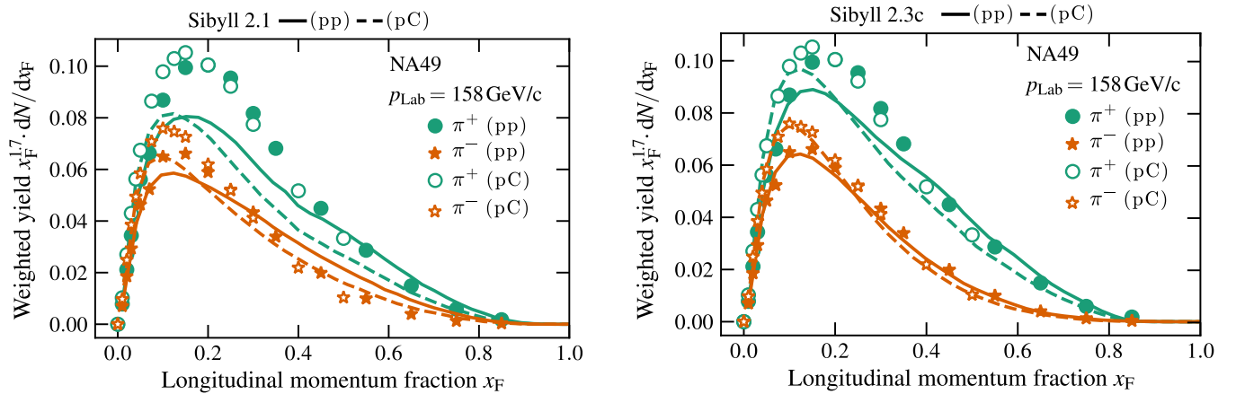
FIG. 12. NA49 pions in SIBYLL-2.1 (left) and SIBYLL-2.3c (right) [35,36] for proton-proton (solid) and proton-carbon (dashed) interactions. In the fragmentation region \pi^+ ( u\bar{d} ) dominate over \pi^- ( d\bar{u} ) because of the quark content of the proton ( uud ). The remnant model in SIBYLL-2.3c is tuned to reproduce these data in the forward region.
