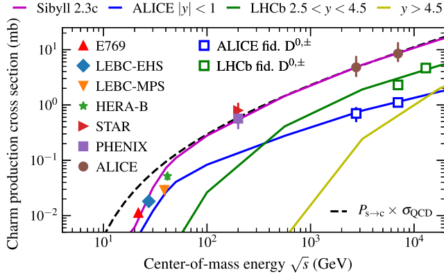
FIG. 20. Inclusive cross section of the production of charmed quarks. Data below 100 GeV are from fixed-target experiments [52–56]. Intermediate and high energy data are from the RHIC and the LHC [57–62]. Apart from the full cross section (magenta line), cross sections for different phase space cuts of the LHC experiments are shown. The blue line corresponds to the central phase space covered in ALICE ( |y| < 0.5 ), while the green line corresponds to the more forward coverage of LHCb ( 2.5 < y < 4.5 ). In yellow the contribution from phase space not covered by any experiment is shown. The dashed line represents the cross section for hard parton scattering scaled to represent charm production in the model.
