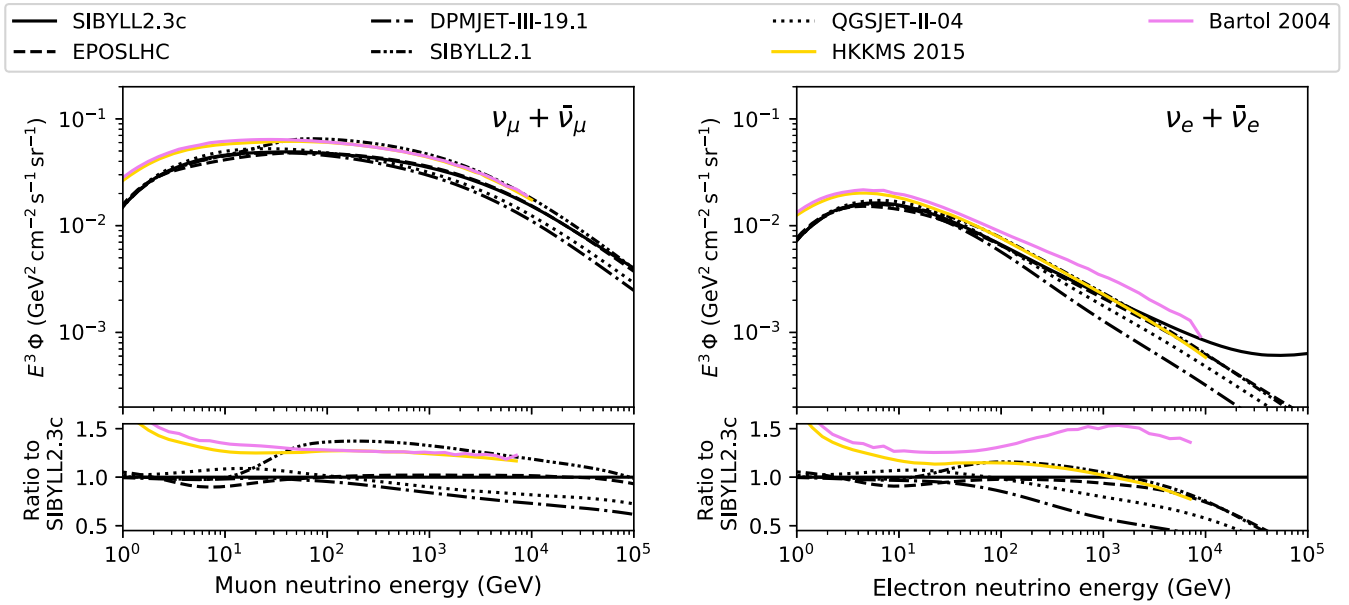
FIG. 34. Figure identical to Figs. 31 and 33 but with the primary flux model from [76] that is used in the HKKMS and Bartol calculations.
