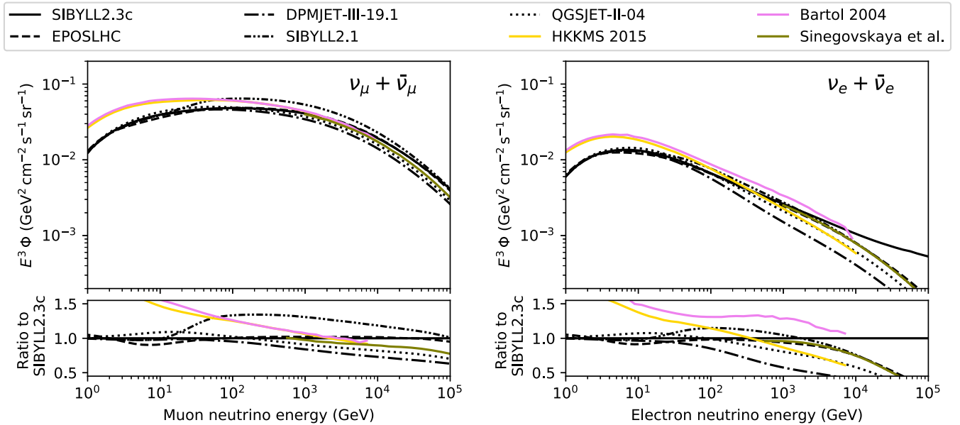
FIG. 31. Atmospheric muon and neutrino fluxes averaged over the zenith angle. The HKKMS and Bartol curves are from computations for Kamioka site and Solar Flux minimum. At energies above a few GeV the dependence on the detector location and solar modulation diminishes. The curves by Sinegovskaya et al. are computed for the similar choice of models as in our case, namely an H3a primary spectrum and QGSJET-II-03 interaction model.
