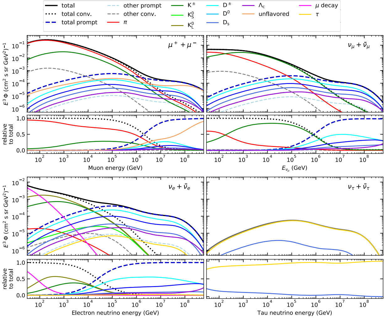
FIG. 5. Contribution from decays of various particles to the atmospheric \mu^+ + \mu^- (top left), \nu_\mu + \bar{\nu}_\mu (top right), \nu_e + \bar{\nu}_e (bottom left) and \nu_\tau + \bar{\nu}_\tau (bottom right) flux in SIBYLL-2.3c and H3a primary model at \theta = 60^\circ .
