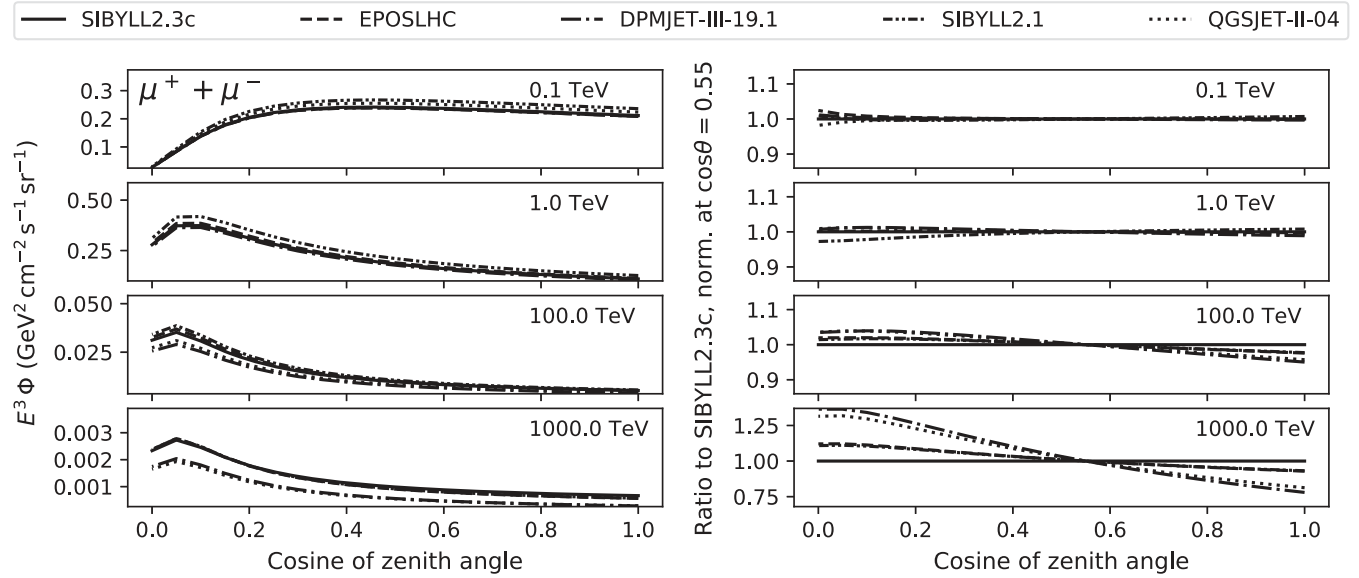
FIG. 36. Azimuth-averaged zenith distributions of the total (conv. + prompt) atmospheric muon flux at high energies. The angle \cos \theta = 0 corresponds to horizontal directions and \cos \theta = 1 to vertical down-going. The left panels show the muon fluxes computed with different hadronic models. Their ratios to SIBYLL-2.3c are located on the right-hand side and normalized to one at \cos \theta = 0.55 . Note the increased scale of the lowest right panel.
