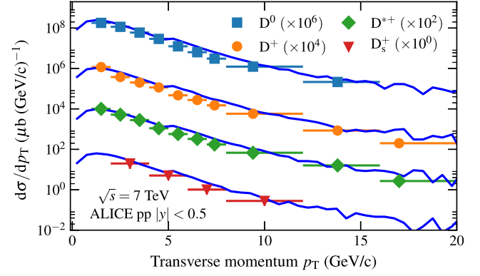
FIG. 22. Spectrum of the transverse momentum of D-mesons. Measurement from ALICE is taken in the central phase space |y| < 0.5 at \sqrt{s} = 7 TeV [60]. Relative abundance of D-mesons, vector resonances ( D^* ) and D-mesons containing a strange quark ( D_s ) is determined by the parameters in the strange quark sector. The line is the prediction from SIBYLL-2.3c.
