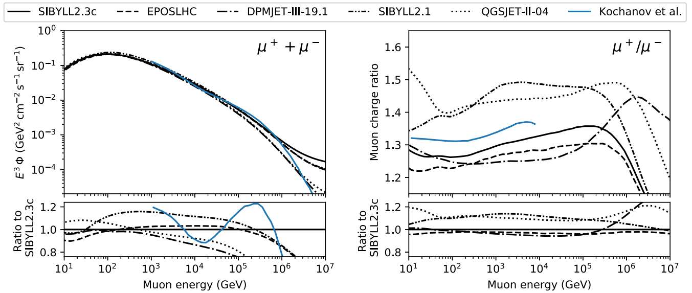
FIG. 30. The atmospheric muon flux and the charge ratio. The MCEQ fluxes for different interaction models are calculated for the zenith angle \theta = 0^\circ and the H3a primary spectrum. For the Kochanov et al. [79] curves the authors used the KM parametrization for hadronic interactions and the Zatsepin-Sokolskaya primary spectrum.
