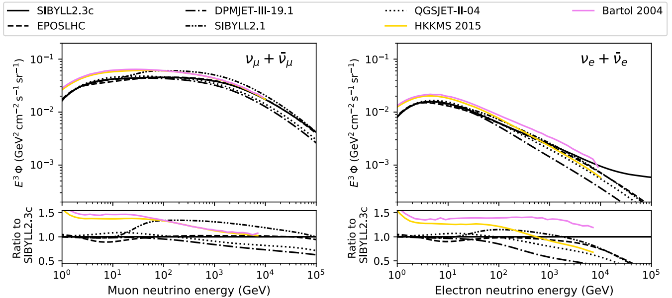
FIG. 33. Atmospheric muon and neutrino fluxes averaged over the zenith angle. The figure is similar to Fig. 31, but instead of the H3a primary flux the nucleon flux from the Global Spline Fit model (GSF) [89] has been used. The differences in the shape and spectral index of the zenith-averaged neutrino flux are significantly reduced in the comparison between MCEQ and the HKKMS or Bartol calculations.
