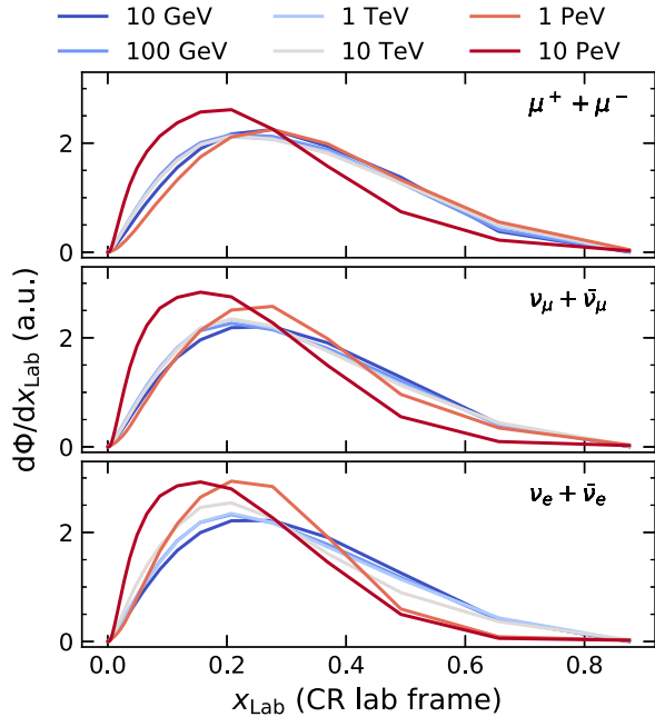
FIG. 11. PDF of the relevant x_{\text{Lab}} values for inclusive leptons at fixed energy. These curves are derived from the inclusive flux, i.e., integrated over the cosmic ray spectrum. An energy independent Z-factor approach would result in a universal shape. Here, the energy dependence comes from deviations from perfect Feynman scaling and from changes in the spectral index of the primary nucleon flux due to the knee and ankle.
