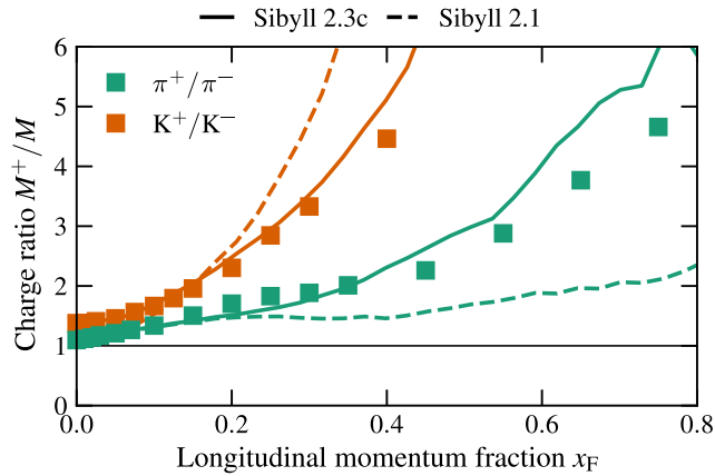
FIG. 14. NA49 measurement of the charge ratio of pions and kaons in pp interactions as a function of Feynman- x [35–37], compared with SIBYLL.
