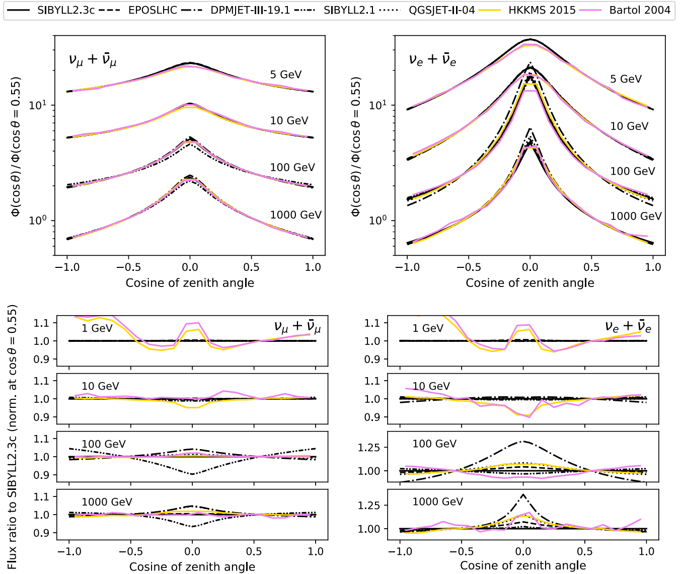
FIG. 35. Azimuth-averaged zenith distributions at fixed neutrino energies. In the upper panels, each individual curve is normalized to one at \cos \theta = 0.55 and offset through a multiplication with 2.5. The lower panels show the model ratios, normalized at \cos \theta = 0.55 to the SIBYLL-2.3c value.
