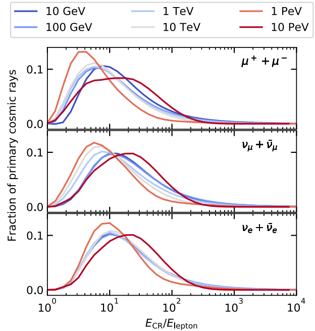
FIG. 4. Like Fig. 3 but as a function of fractional energy E_{\text{cosmic ray}}/E_{\text{lepton}} , for muons (upper panel), muon neutrinos (middle panel) and electron neutrinos (lower panel).
