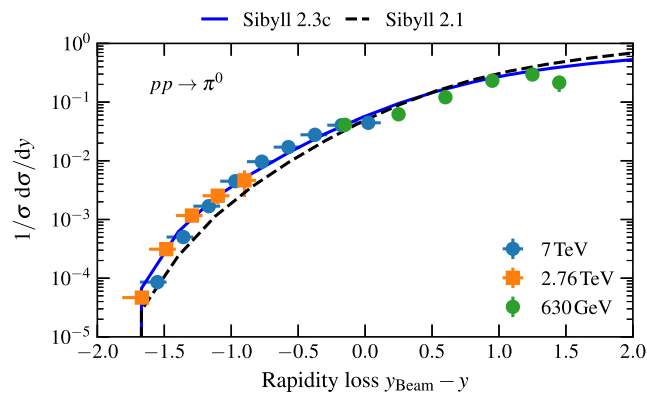
FIG. 16. Yield of neutral pions as a function of the rapidity loss y_{\text{loss}} = y_{\text{beam}} - y at different c.m. energies [38,39]. If Feynman scaling holds in the fragmentation region, the spectrum is universal.
