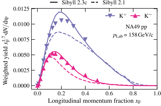
FIG. 13. Longitudinal momentum spectrum of charged kaons measured in pp fixed-target collisions by NA49 [37], compared with SIBYLL.
