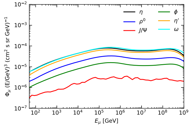
FIG. 6. Breakdown of the unflavored component of the prompt muon flux.
