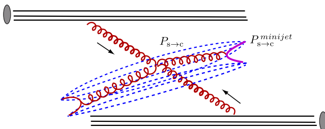
FIG. 18. String configuration for minijets in SIBYLL.
