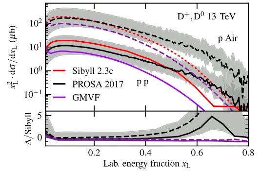
FIG. 27. Comparison of the energy spectra of charmed mesons between SIBYLL (red lines) and NLO QCD calculations [PROSA 2017 [69] (black lines) and GMVF [70] (purple lines)]. Energy is evaluated in the lab. frame. The lower panel shows the difference relative to SIBYLL. The grey band represents the theoretical uncertainty in the PROSA calculation (factorization and renormalization scale). Calculations for pp interactions are shown by solid lines and those for p-air with are dashed or dotted. The NLO calculations for an Air target are scaled up according to 14.5 \times pp .
