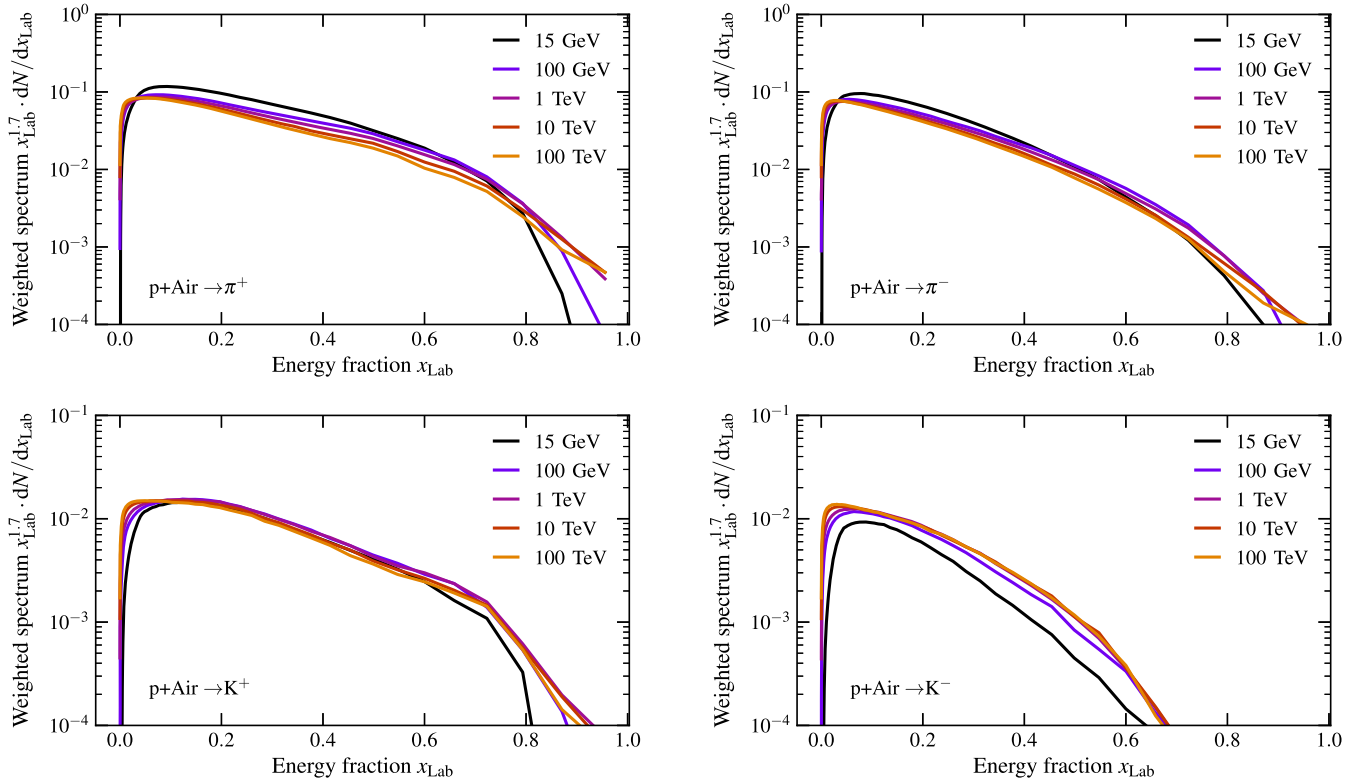
FIG. 17. Scaling behavior of the energy distribution of secondary mesons in SIBYLL-2.3c. For perfect scaling the lines for the different laboratory frame projectile energies should be on top of each other. The lowest energy line deviates due to threshold. At very small x_{\text{Lab}} scaling violations due to multiparton interactions are expected and visible at higher energies. For \pi^- and K^- the scaling is better than for their positively charged counterparts, which are more affected by the remnant model.
