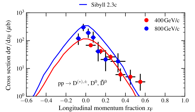
FIG. 23. Feynman- x spectrum of charmed mesons in pp interactions. Data are from LEBC experiment [54,64], recorded at beam momenta of 400 and 800 GeV/c. The lines are the predictions from SIBYLL-2.3c.
