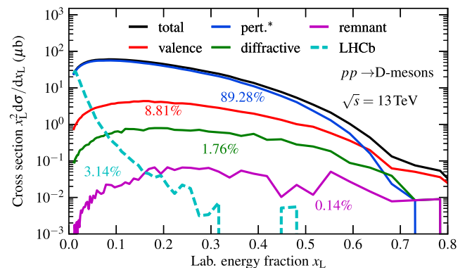
FIG. 28. Weighted energy spectrum of D-mesons at \sqrt{s} = 13 TeV. The energy of the particles is taken in the lab. frame and expressed relative to the beam energy. Contributions by different phase space intervals are shown. The contribution of the phase space covered by LHCb in events that also trigger LHCb is around 3%.
