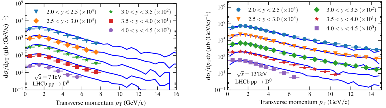
FIG. 24. p_T -spectrum of neutral D-mesons in LHCb at 7 and 13 TeV c.m. energy [61,62] compared to SIBYLL 2.3c
