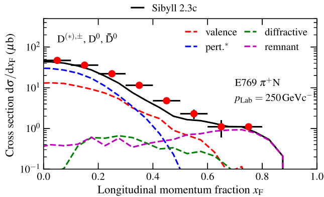
FIG. 21. Feynman- x spectrum of charmed mesons in \pi -nucleus interactions. Data are from E769 [63], taken with beam momentum of 250 GeV/c. Dashed lines are contributions from individual processes in SIBYLL. The “remnant” contribution arises from the exchange of a quark with the soft strings (see Fig. 19).
