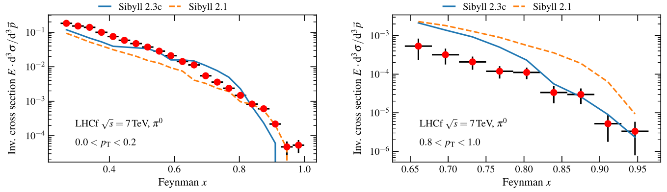
FIG. 15. Longitudinal momentum spectrum of the of neutral pions at 7 TeV. Data are from the LHCf spectrometer, covering 8.9 < \eta < 10.2 in two different p_T bins.
