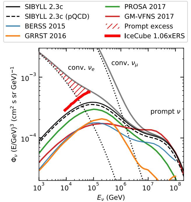
FIG. 32. Prompt atmospheric muon and electron neutrino fluxes averaged over zenith angles. All fluxes are computed for the H3a cosmic ray flux model and the most differences arise from the charm cross section calculations. SIBYLL-2.3c (pQCD) is the component attributed to the perturbative* component from Figs. 28 and 27. The pQCD calculations BERSS [84], GRRST [65,87], PROSA [69] and GM-VNFS [70] are computed at NLO precision under different assumptions for vertical angles. For \theta = 0^\circ the shape of the black curves would coincide with the shape of the green curve. They are accompanied by large error bands which are omitted for clarity. Within the errors all models are compatible with each other. The bound by IceCube [86] of 1.06x is expressed in units of normalization of the model from [88], recomputed for the H3a primary flux. The red hatched patch represents the excess of the prompt flux that leads to distinct signatures in the \nu_\mu/\nu_e and the vertical-to-horizontal ratio.
