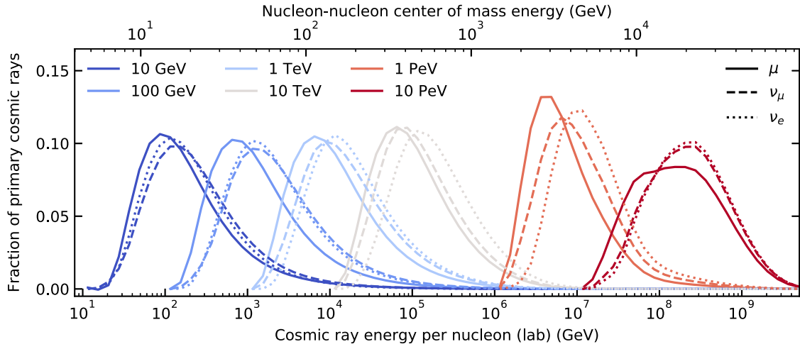
FIG. 3. Probability density functions (PDFs) of the primary nucleon energies corresponding to inclusive leptons at a fixed energy (colors). The solid, dashed and dotted lines refer to the individual lepton species. Atmospheric neutrinos up to 1 PeV probe center of mass collisions (top axis) that are within reach of current collider experiments (the LHC reaches 13 TeV).
