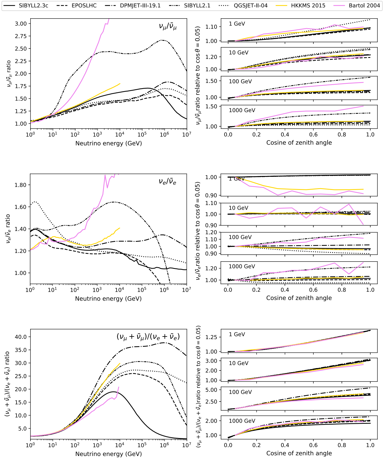
FIG. 37. Neutrino-antineutrino and flavor ratios. The left panels show zenith-averaged distributions. The right panels demonstrate the relative zenith angle dependence of each ratio for a fixed neutrino energy. These curves are normalized such that at \cos\theta = 0.05 the value is one. Note that the axes scales for the right panels were allowed to float.
