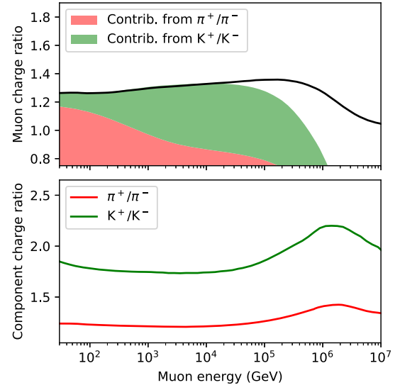
FIG. 7. Muons charge ratio and effective components from pion and kaon decays. (Upper panel) The solid line is the total muon charge ratio from SIBYLL and the areas the individual weights from the pion and kaon component. (Lower panel) The colored areas are a measure of the effective weight of the pion and the kaon component. The variations at 1 PeV come from the change of the spectral index at the knee, resulting in a different weight (or mean) of the x_{\text{Lab}} distribution of secondaries.
