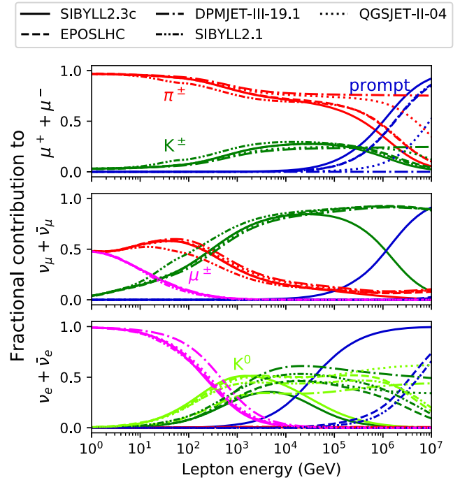
FIG. 29. Fractions of hadrons decaying into atmospheric leptons. The muon flux (upper panel) is calculated with the indicated interaction models for \theta = 0^\circ . The neutrino fluxes (lower panels) show the results for zenith averaged fluxes.
