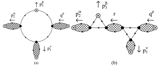
Figure 3. The two classes of diagrams contributing to HLbL in the ENJL model. The crossed regions indicate the bubble sum “propagators.” (a) Quark-loop type (b) Resonance exchange type
