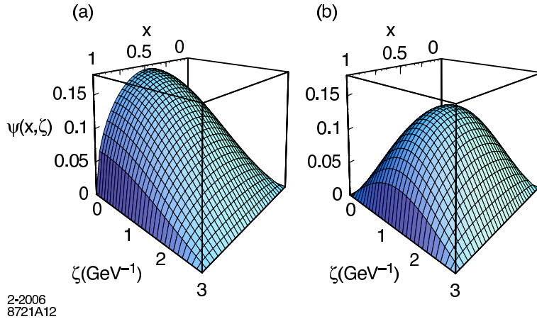
FIG. 1: Two-parton bound state holographic LFWF \tilde{\psi}(x, \zeta) for \Lambda_{\text{QCD}} = 0.32 GeV: (a) ground state L = 0 , k = 1 , (b) first orbital excited state L = 1 , k = 1 .
